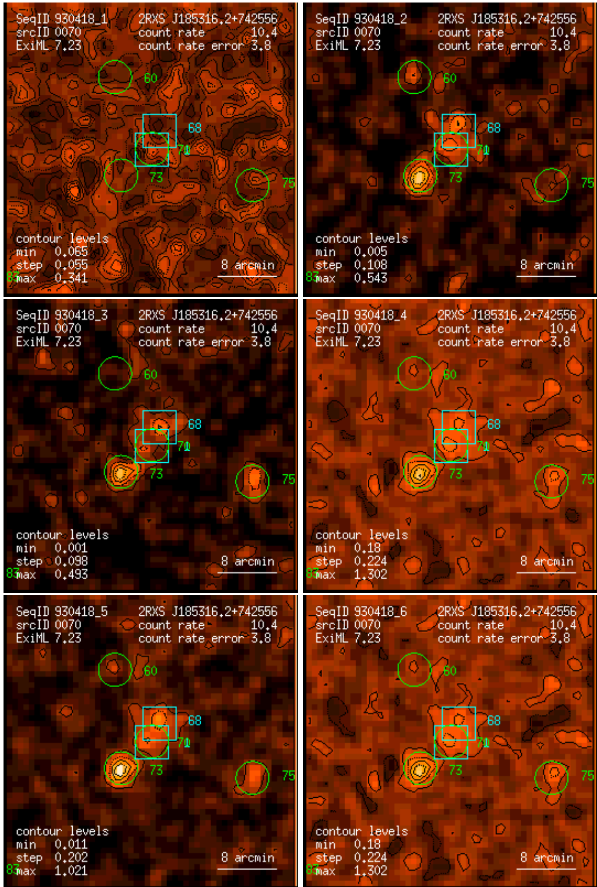
Figure 70: RASS 930418: detection 0070: band rate images, Gaussian filter: (1) PSPC channels 11 – 41, (2) 52 – 90, (3) 91 – 201, (4) 11 – 235, (5) 52 – 201, (6) 11 – 201. Broad band rates in counts/ks. Band rate contour levels in counts/ks/arcmin 2 .
