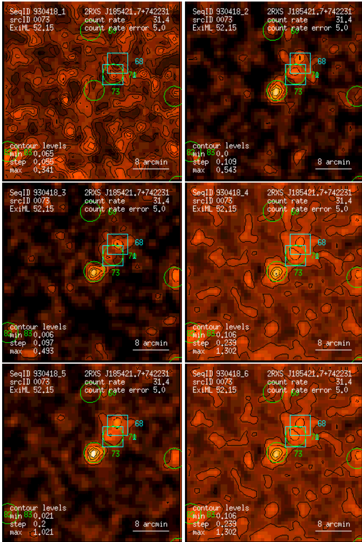
Figure 73: RASS 930418: detection 0073: band rate images, Gaussian filter: (1) PSPC channels 11 – 41, (2) 52 – 90, (3) 91 – 201, (4) 11 – 235, (5) 52 – 201, (6) 11 – 201. Broad band rates in counts/ks. Band rate contour levels in counts/ks/arcmin 2 .
