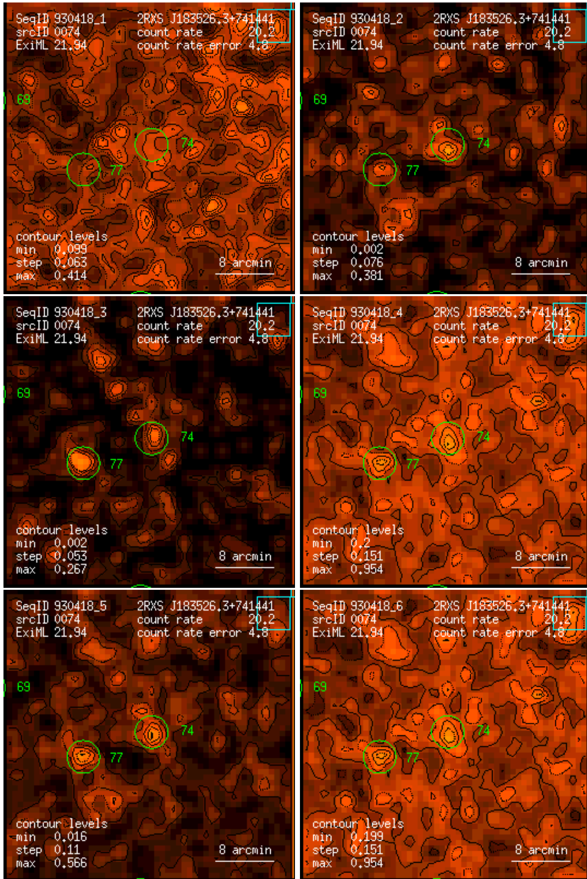
Figure 74: RASS 930418: detection 0074: band rate images, Gaussian filter: (1) PSPC channels 11 – 41, (2) 52 – 90, (3) 91 – 201, (4) 11 – 235, (5) 52 – 201, (6) 11 – 201. Broad band rates in counts/ks. Band rate contour levels in counts/ks/arcmin 2 .
