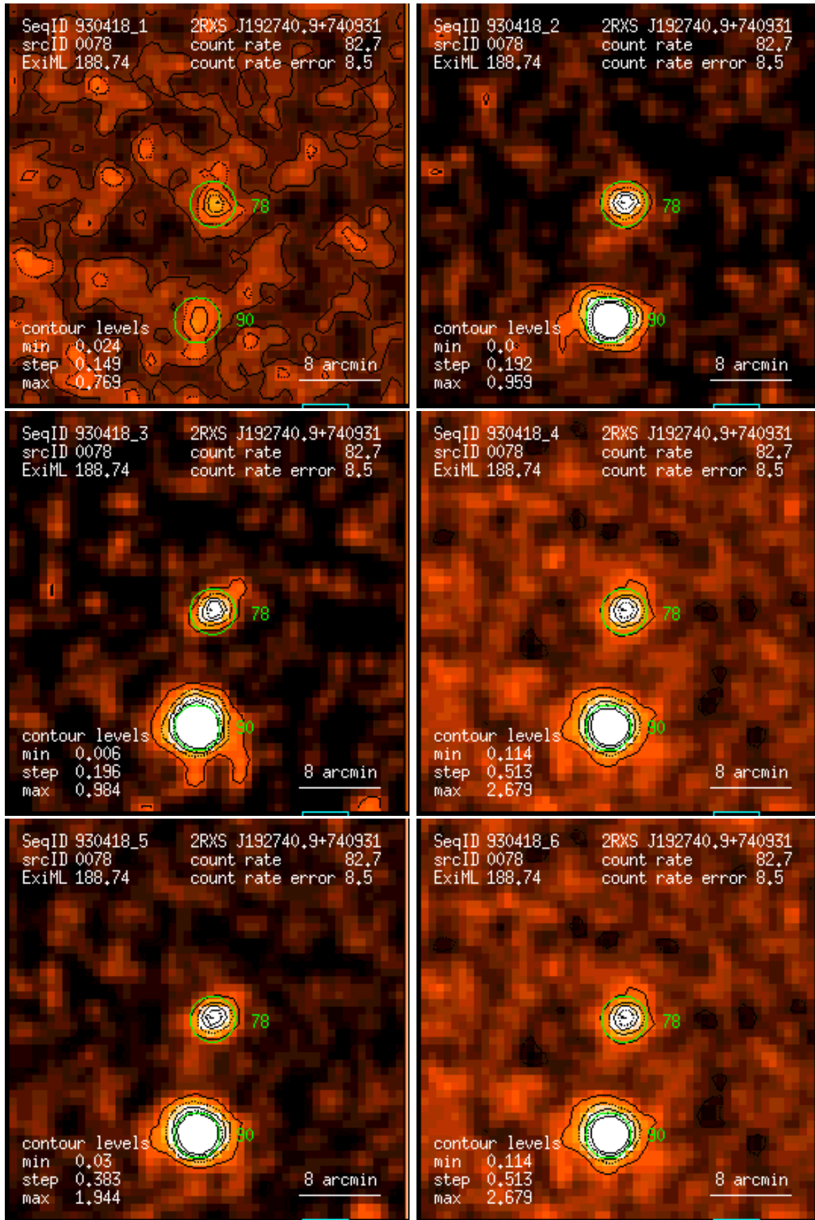
Figure 78: RASS 930418: detection 0078: band rate images, Gaussian filter: (1) PSPC channels 11 – 41, (2) 52 – 90, (3) 91 – 201, (4) 11 – 235, (5) 52 – 201, (6) 11 – 201. Broad band rates in counts/ks. Band rate contour levels in counts/ks/arcmin 2 .
