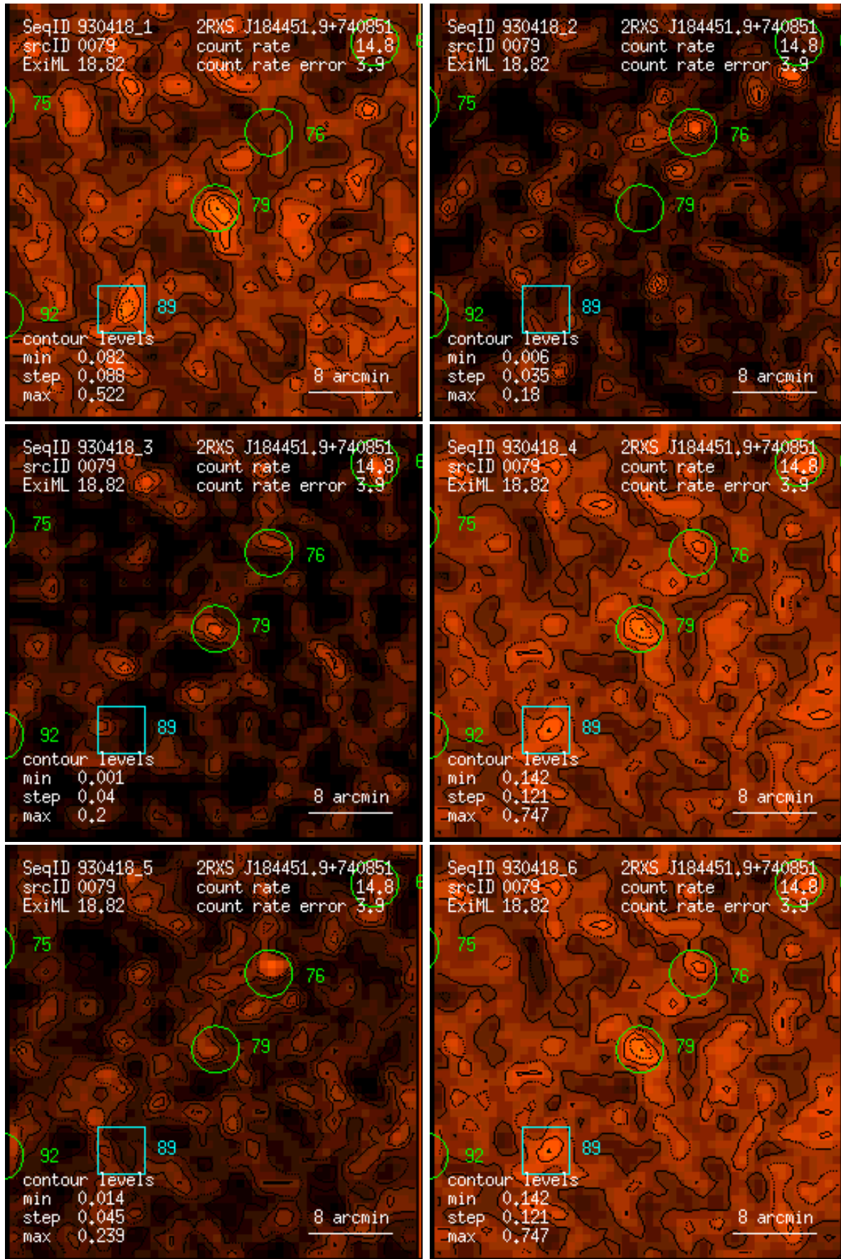
Figure 79: RASS 930418: detection 0079: band rate images, Gaussian filter: (1) PSPC channels 11 – 41, (2) 52 – 90, (3) 91 – 201, (4) 11 – 235, (5) 52 – 201, (6) 11 – 201. Broad band rates in counts/ks. Band rate contour levels in counts/ks/arcmin 2 .
