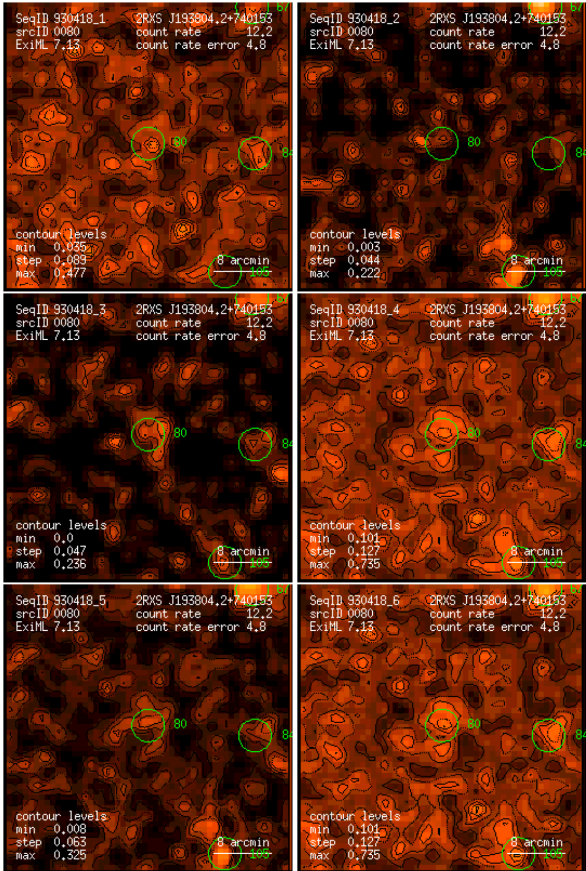
Figure 80: RASS 930418: detection 0080: band rate images, Gaussian filter: (1) PSPC channels 11 – 41, (2) 52 – 90, (3) 91 – 201, (4) 11 – 235, (5) 52 – 201, (6) 11 – 201. Broad band rates in counts/ks. Band rate contour levels in counts/ks/arcmin 2 .
