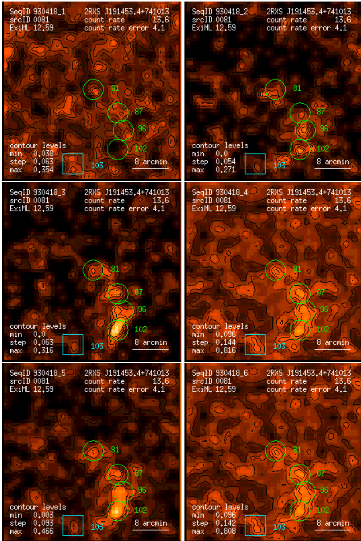
Figure 81: RASS 930418: detection 0081: band rate images, Gaussian filter: (1) PSPC channels 11 – 41, (2) 52 – 90, (3) 91 – 201, (4) 11 – 235, (5) 52 – 201, (6) 11 – 201. Broad band rates in counts/ks. Band rate contour levels in counts/ks/arcmin 2 .
