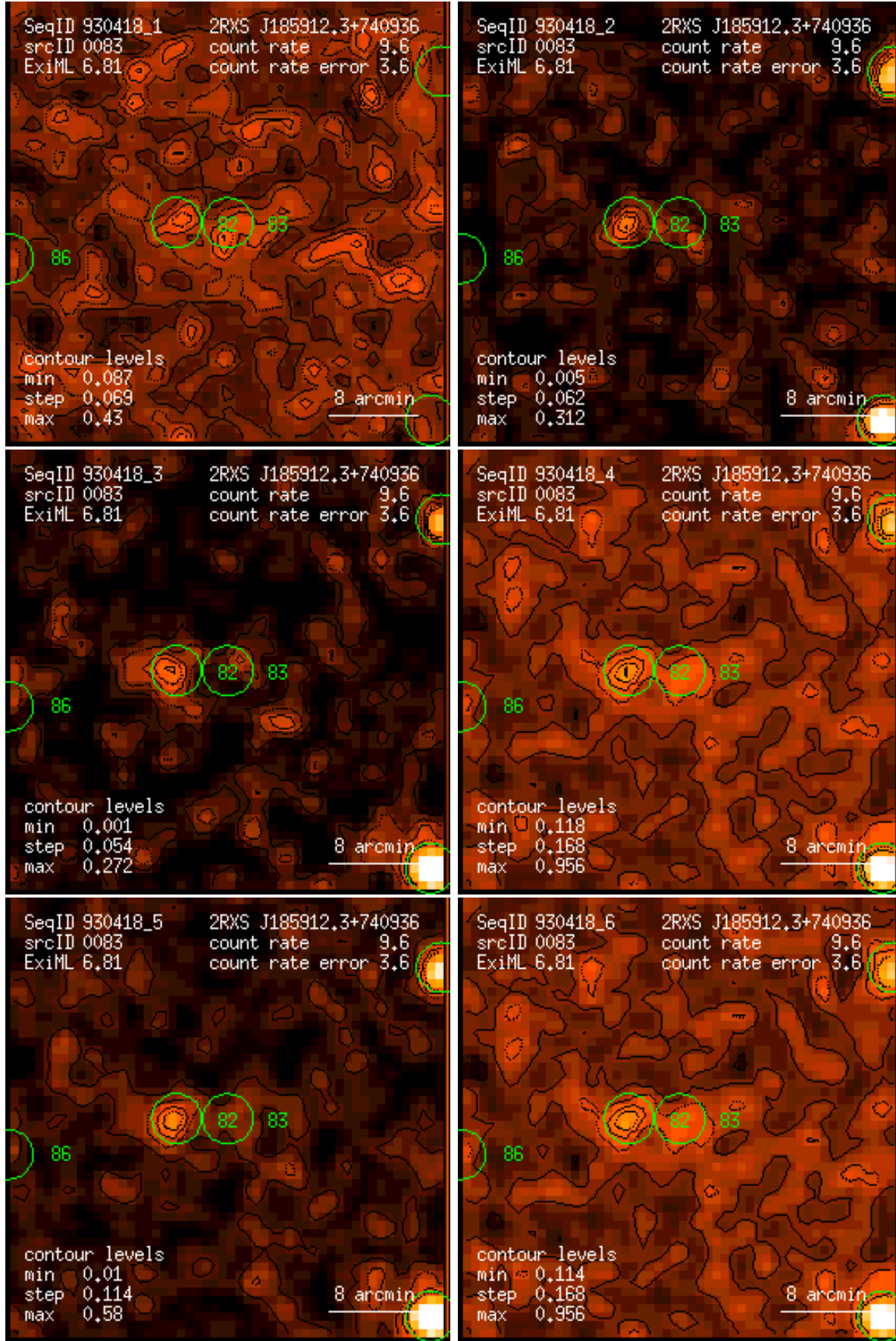
Figure 83: RASS 930418: detection 0083: band rate images, Gaussian filter: (1) PSPC channels 11 – 41, (2) 52 – 90, (3) 91 – 201, (4) 11 – 235, (5) 52 – 201, (6) 11 – 201. Broad band rates in counts/ks. Band rate contour levels in counts/ks/arcmin 2 .
