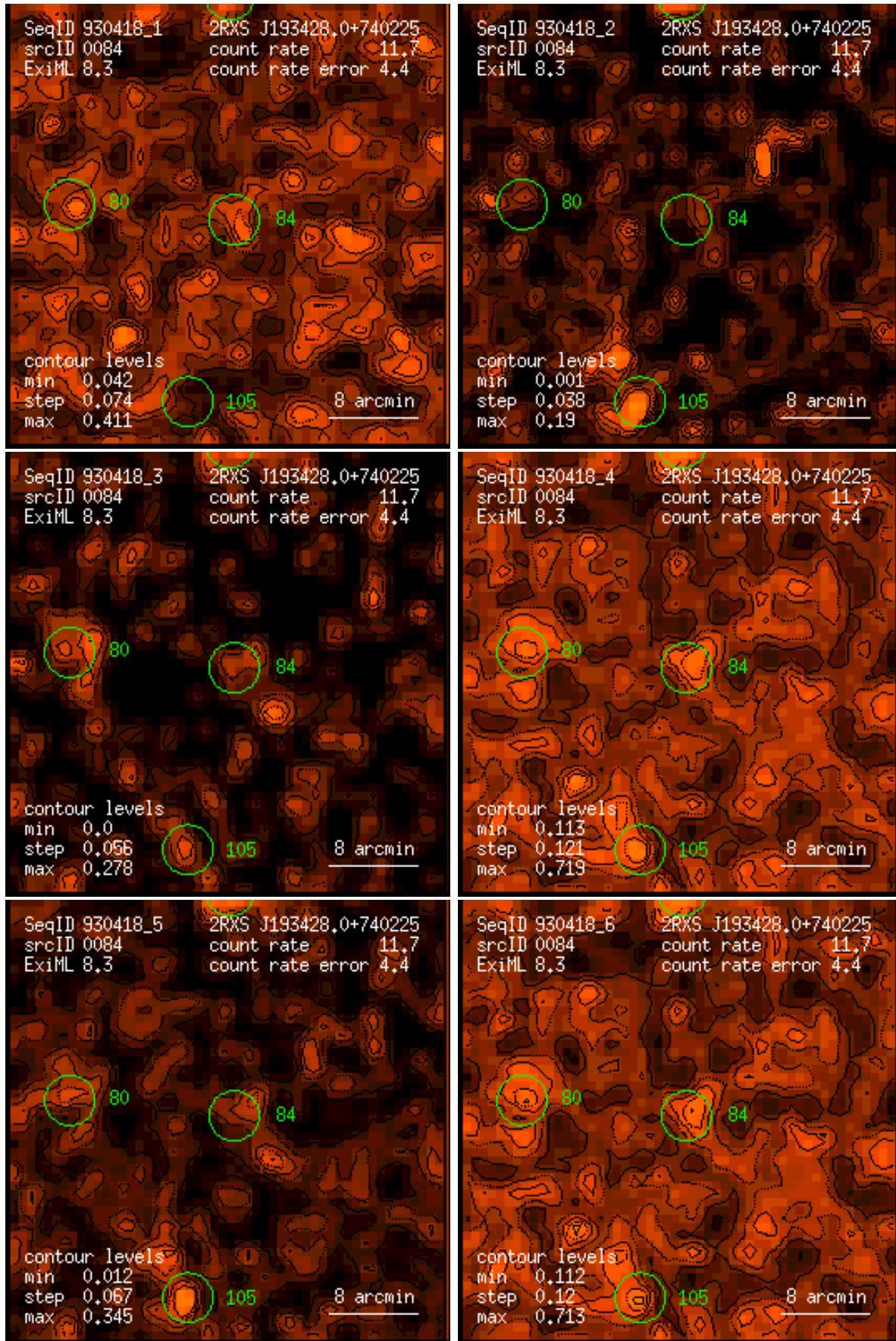
Figure 84: RASS 930418: detection 0084: band rate images, Gaussian filter: (1) PSPC channels 11 – 41, (2) 52 – 90, (3) 91 – 201, (4) 11 – 235, (5) 52 – 201, (6) 11 – 201. Broad band rates in counts/ks. Band rate contour levels in counts/ks/arcmin 2 .
