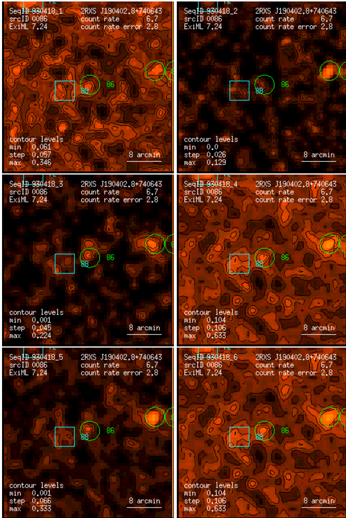
Figure 86: RASS 930418: detection 0086: band rate images, Gaussian filter: (1) PSPC channels 11 – 41, (2) 52 – 90, (3) 91 – 201, (4) 11 – 235, (5) 52 – 201, (6) 11 – 201. Broad band rates in counts/ks. Band rate contour levels in counts/ks/arcmin 2 .
