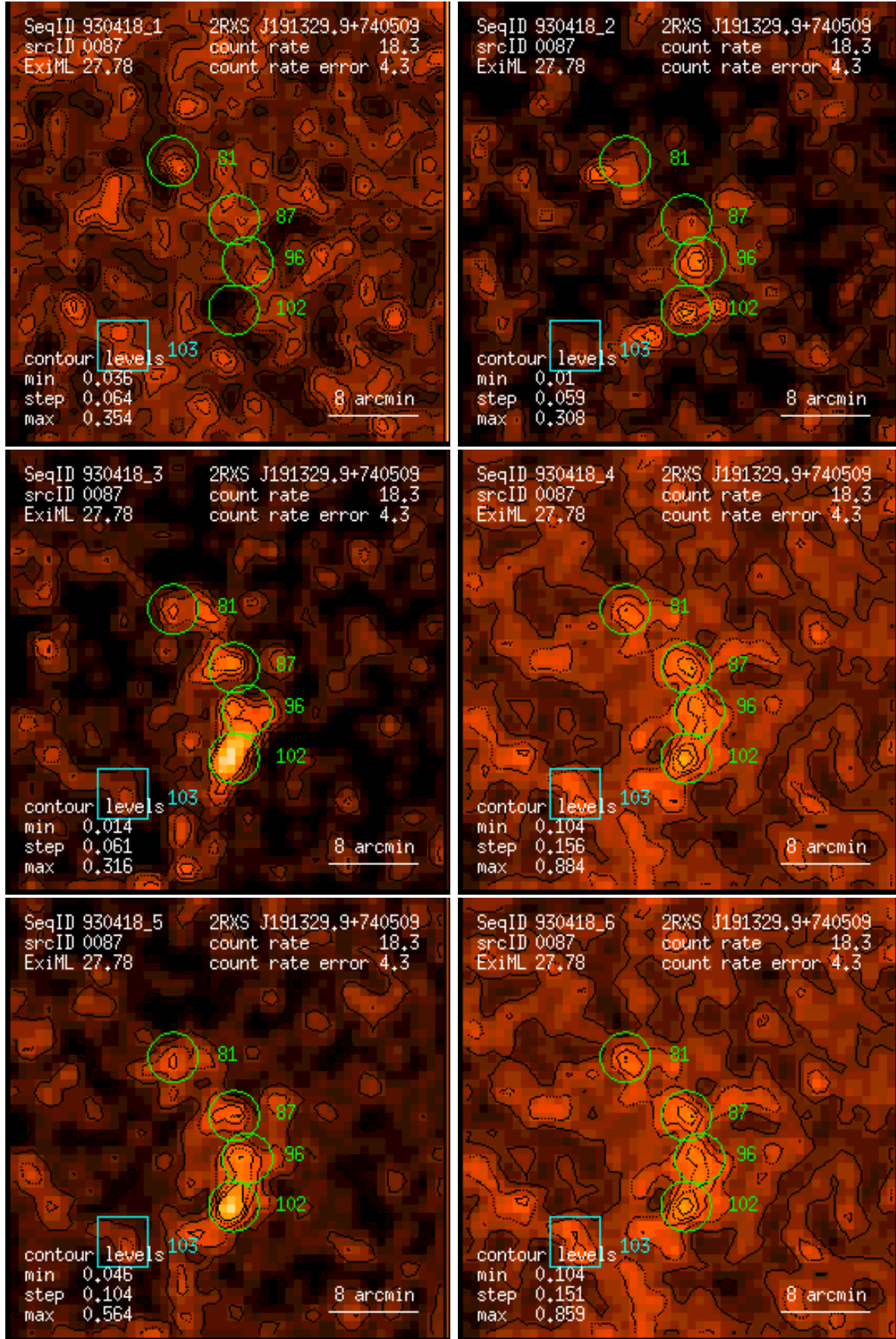
Figure 87: RASS 930418: detection 0087: band rate images, Gaussian filter: (1) PSPC channels 11 – 41, (2) 52 – 90, (3) 91 – 201, (4) 11 – 235, (5) 52 – 201, (6) 11 – 201. Broad band rates in counts/ks. Band rate contour levels in counts/ks/arcmin 2 .
