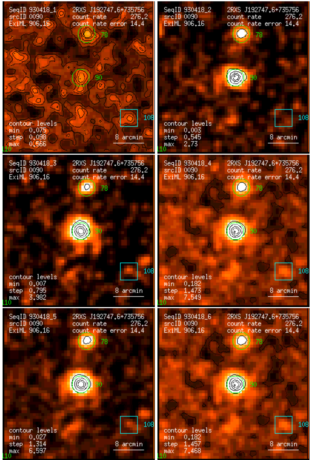
Figure 90: RASS 930418: detection 0090: band rate images, Gaussian filter: (1) PSPC channels 11 – 41, (2) 52 – 90, (3) 91 – 201, (4) 11 – 235, (5) 52 – 201, (6) 11 – 201. Broad band rates in counts/ks. Band rate contour levels in counts/ks/arcmin 2 .
