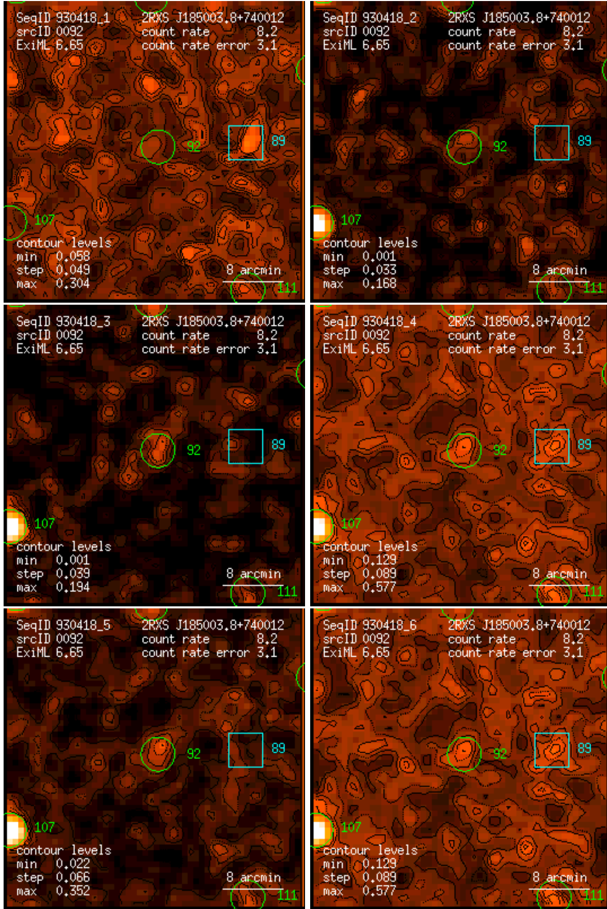
Figure 92: RASS 930418: detection 0092: band rate images, Gaussian filter: (1) PSPC channels 11 – 41, (2) 52 – 90, (3) 91 – 201, (4) 11 – 235, (5) 52 – 201, (6) 11 – 201. Broad band rates in counts/ks. Band rate contour levels in counts/ks/arcmin 2 .
