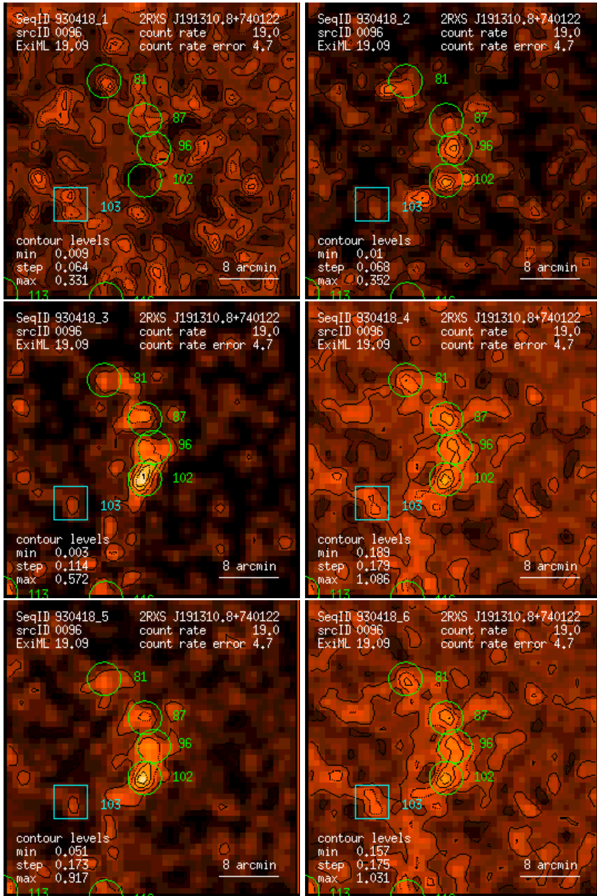
Figure 96: RASS 930418: detection 0096: band rate images, Gaussian filter: (1) PSPC channels 11 – 41, (2) 52 – 90, (3) 91 – 201, (4) 11 – 235, (5) 52 – 201, (6) 11 – 201. Broad band rates in counts/ks. Band rate contour levels in counts/ks/arcmin 2 .
