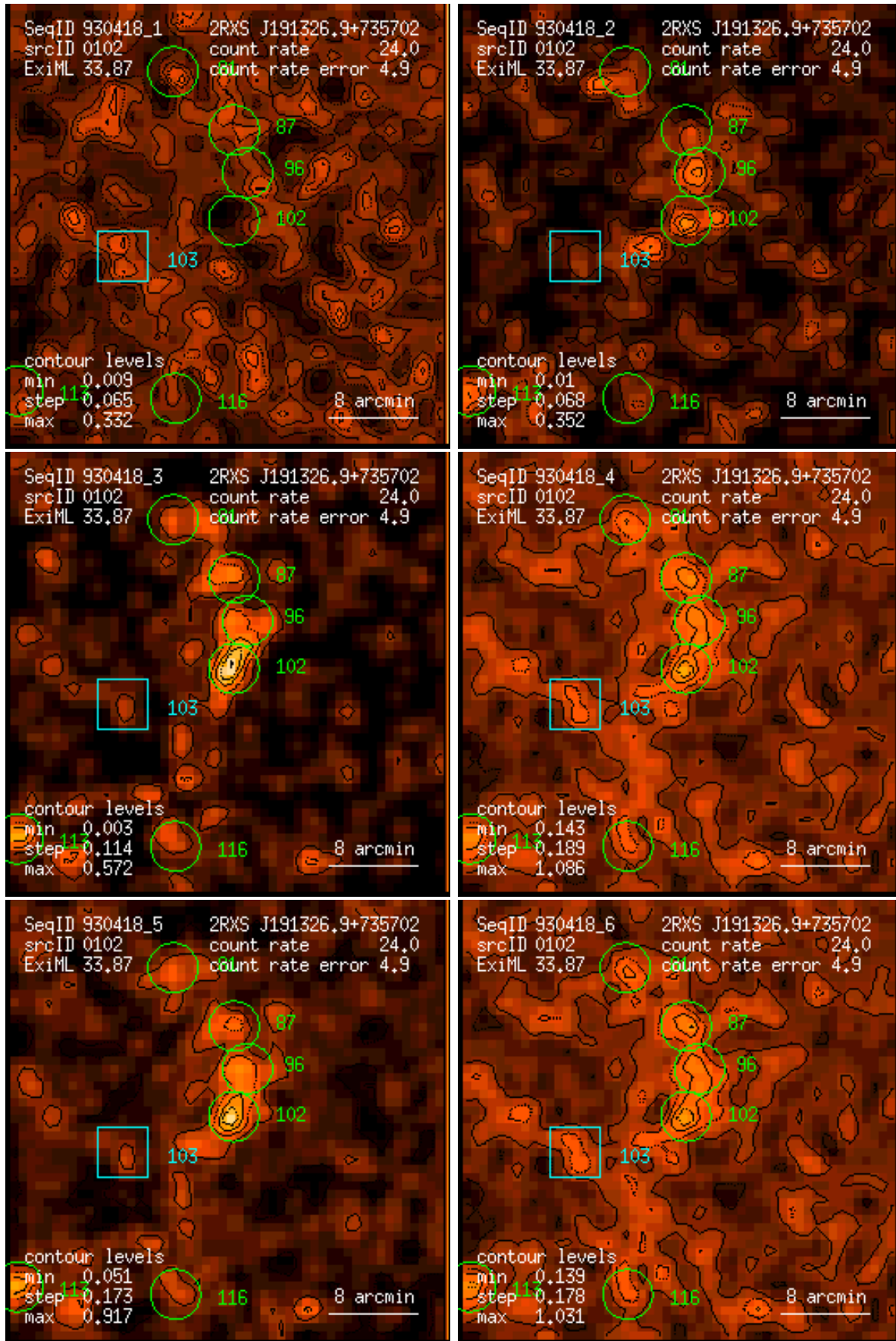
Figure 102: RASS 930418: detection 0102: band rate images, Gaussian filter: (1) PSPC channels 11 – 41, (2) 52 – 90, (3) 91 – 201, (4) 11 – 235, (5) 52 – 201, (6) 11 – 201. Broad band rates in counts/ks. Band rate contour levels in counts/ks/arcmin 2 .
