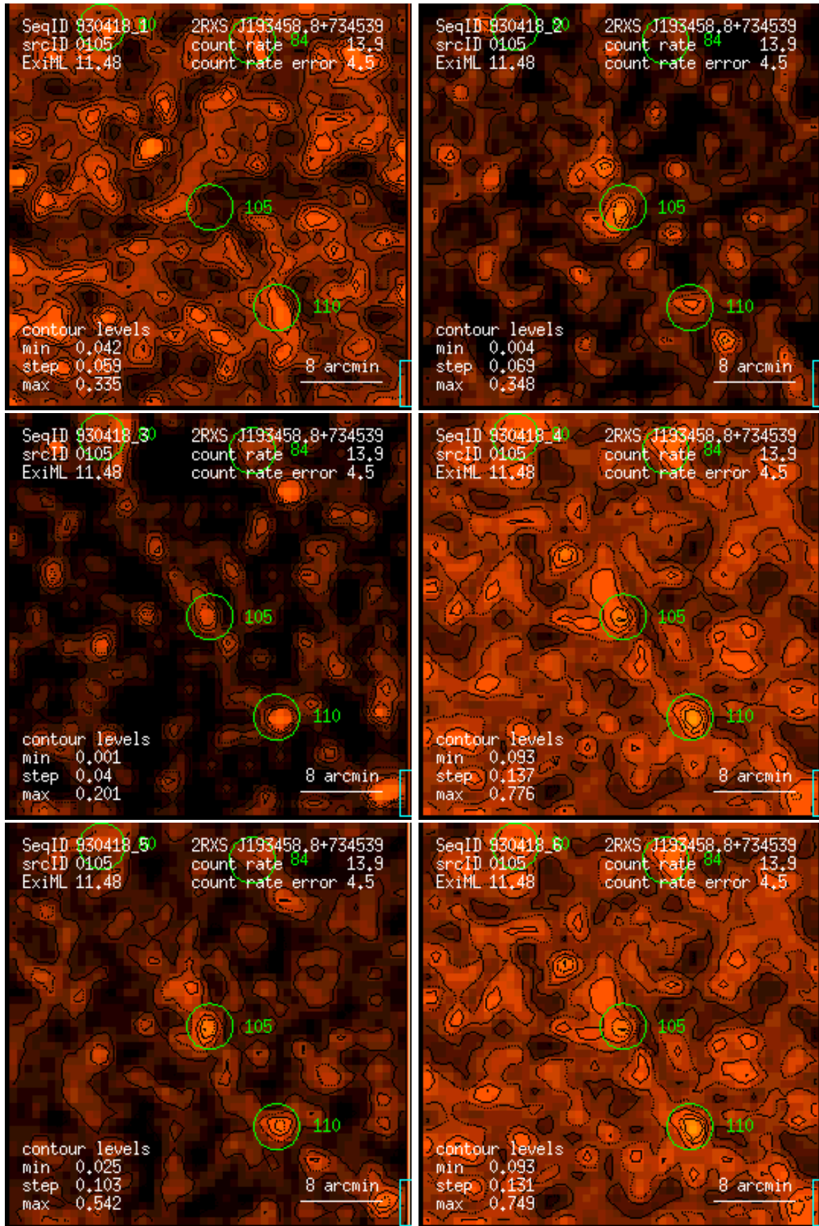
Figure 105: RASS 930418: detection 0105: band rate images, Gaussian filter: (1) PSPC channels 11 – 41, (2) 52 – 90, (3) 91 – 201, (4) 11 – 235, (5) 52 – 201, (6) 11 – 201. Broad band rates in counts/ks. Band rate contour levels in counts/ks/arcmin 2 .
