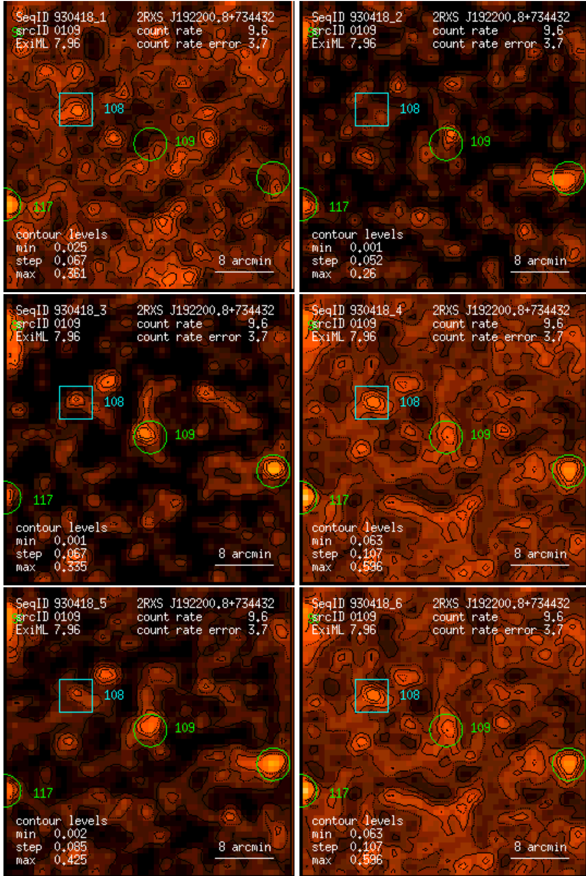
Figure 109: RASS 930418: detection 0109: band rate images, Gaussian filter: (1) PSPC channels 11 – 41, (2) 52 – 90, (3) 91 – 201, (4) 11 – 235, (5) 52 – 201, (6) 11 – 201. Broad band rates in counts/ks. Band rate contour levels in counts/ks/arcmin 2 .
