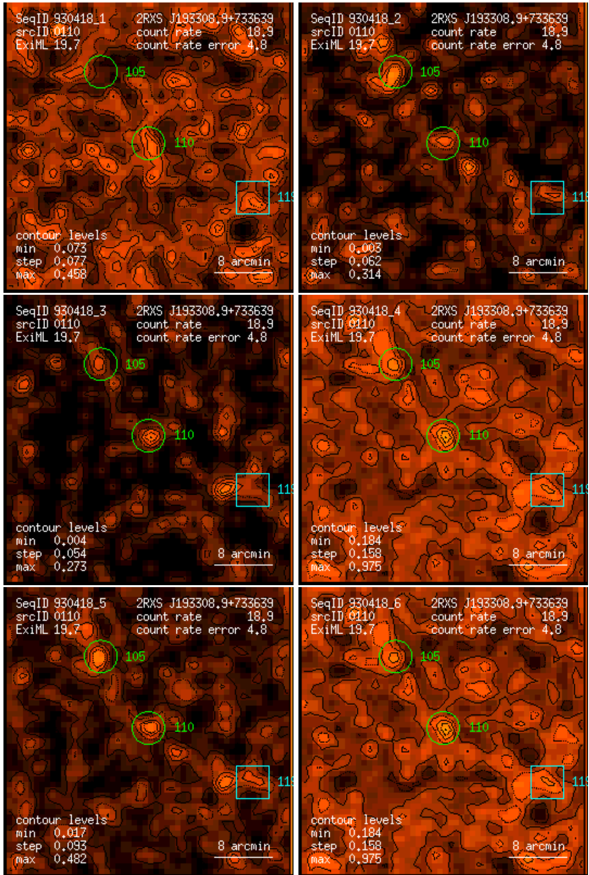
Figure 110: RASS 930418: detection 0110: band rate images, Gaussian filter: (1) PSPC channels 11 – 41, (2) 52 – 90, (3) 91 – 201, (4) 11 – 235, (5) 52 – 201, (6) 11 – 201. Broad band rates in counts/ks. Band rate contour levels in counts/ks/arcmin 2 .
