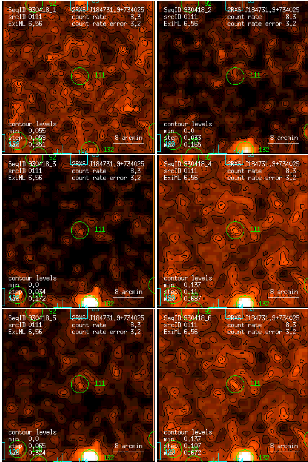
Figure 111: RASS 930418: detection 0111: band rate images, Gaussian filter: (1) PSPC channels 11 – 41, (2) 52 – 90, (3) 91 – 201, (4) 11 – 235, (5) 52 – 201, (6) 11 – 201. Broad band rates in counts/ks. Band rate contour levels in counts/ks/arcmin 2 .
