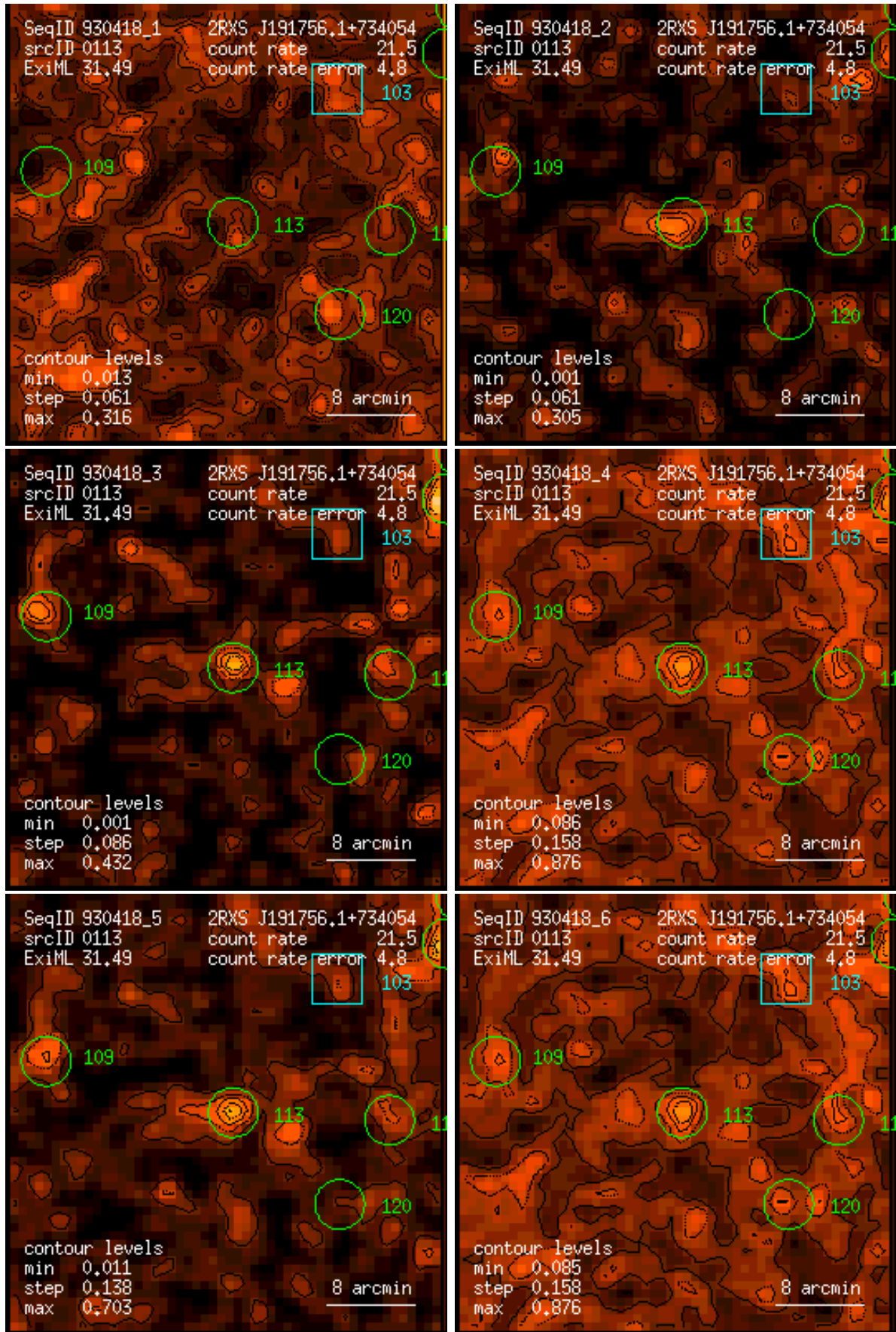
Figure 113: RASS 930418: detection 0113: band rate images, Gaussian filter: (1) PSPC channels 11 – 41, (2) 52 – 90, (3) 91 – 201, (4) 11 – 235, (5) 52 – 201, (6) 11 – 201. Broad band rates in counts/ks. Band rate contour levels in counts/ks/arcmin 2 .
