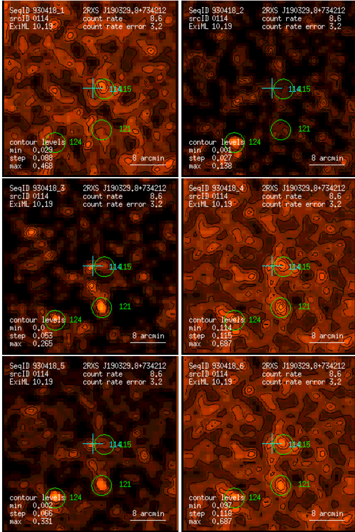
Figure 114: RASS 930418: detection 0114: band rate images, Gaussian filter: (1) PSPC channels 11 – 41, (2) 52 – 90, (3) 91 – 201, (4) 11 – 235, (5) 52 – 201, (6) 11 – 201. Broad band rates in counts/ks. Band rate contour levels in counts/ks/arcmin 2 .
