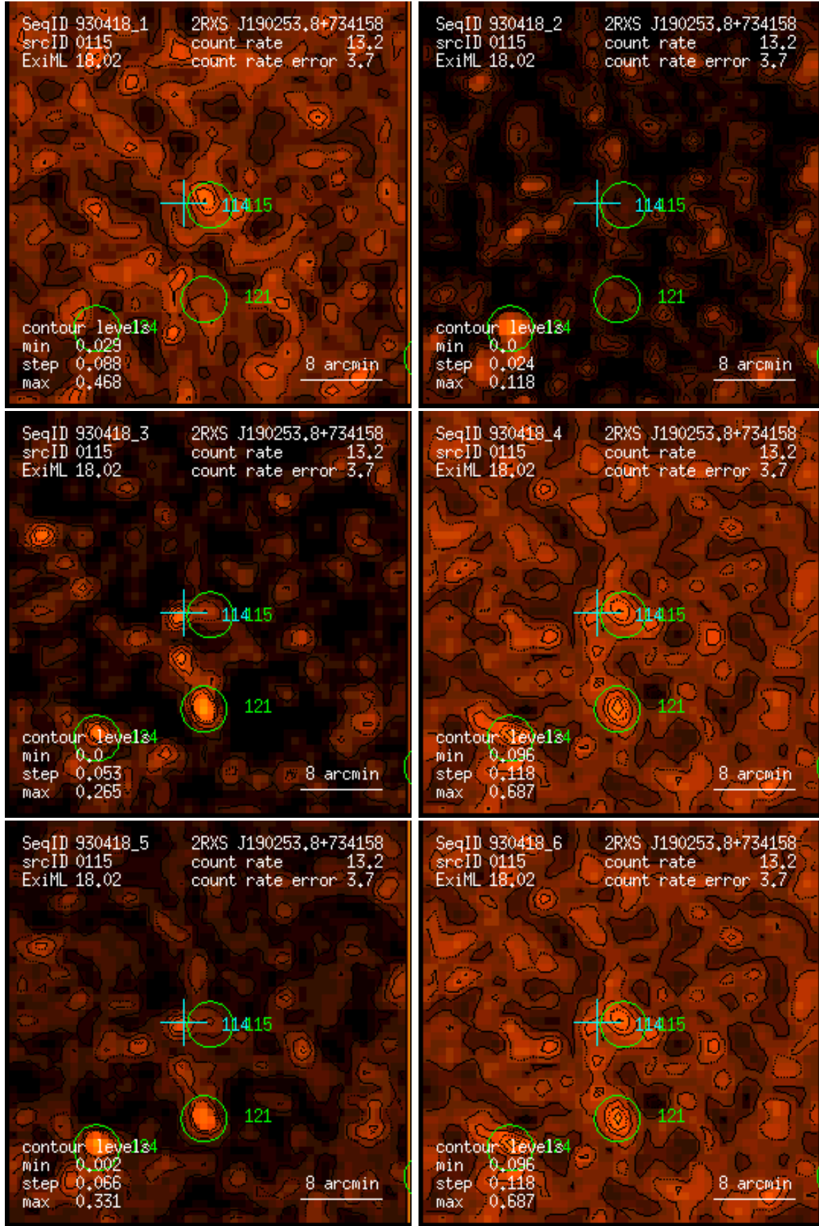
Figure 115: RASS 930418: detection 0115: band rate images, Gaussian filter: (1) PSPC channels 11 – 41, (2) 52 – 90, (3) 91 – 201, (4) 11 – 235, (5) 52 – 201, (6) 11 – 201. Broad band rates in counts/ks. Band rate contour levels in counts/ks/arcmin 2 .
