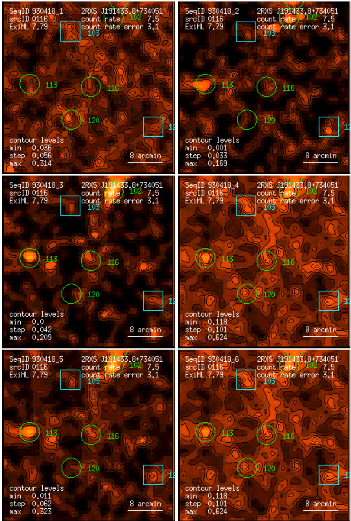
Figure 116: RASS 930418: detection 0116: band rate images, Gaussian filter: (1) PSPC channels 11 – 41, (2) 52 – 90, (3) 91 – 201, (4) 11 – 235, (5) 52 – 201, (6) 11 – 201. Broad band rates in counts/ks. Band rate contour levels in counts/ks/arcmin 2 .
