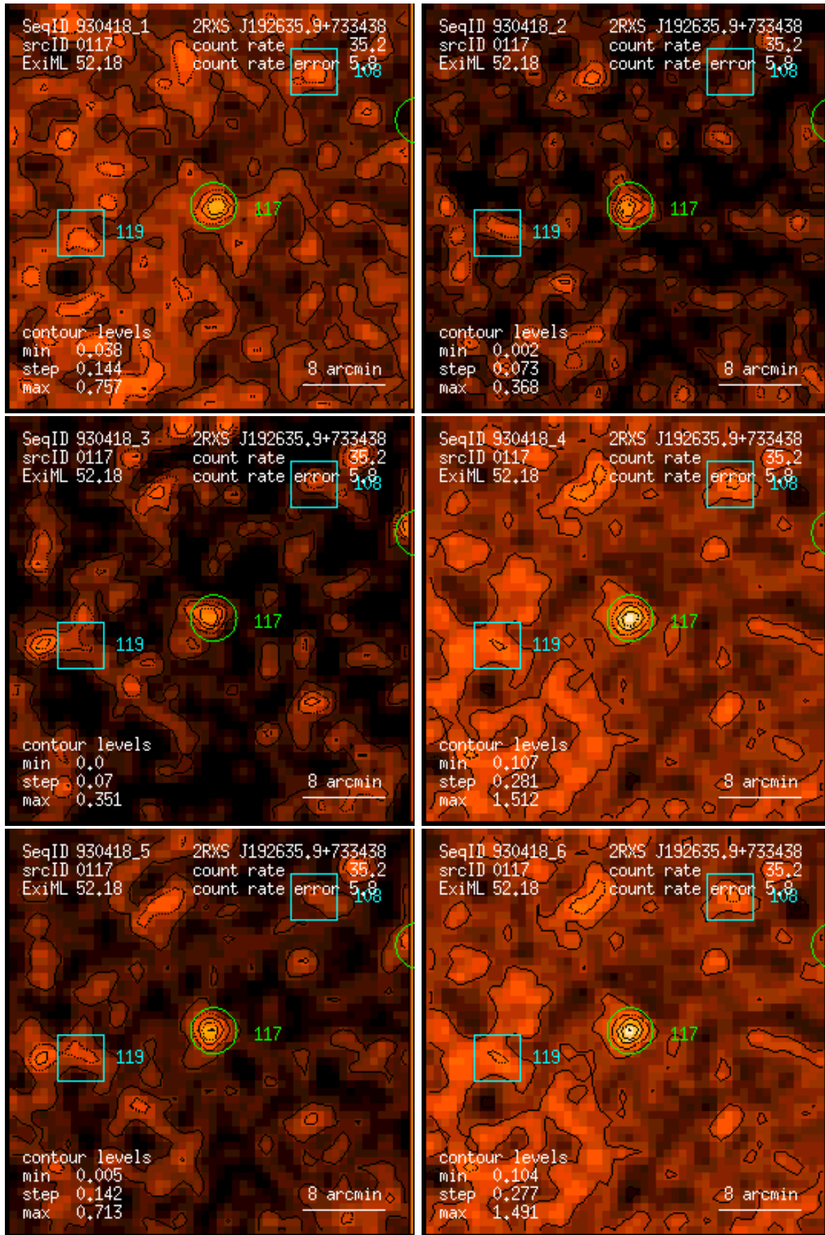
Figure 117: RASS 930418: detection 0117: band rate images, Gaussian filter: (1) PSPC channels 11 – 41, (2) 52 – 90, (3) 91 – 201, (4) 11 – 235, (5) 52 – 201, (6) 11 – 201. Broad band rates in counts/ks. Band rate contour levels in counts/ks/arcmin 2 .
