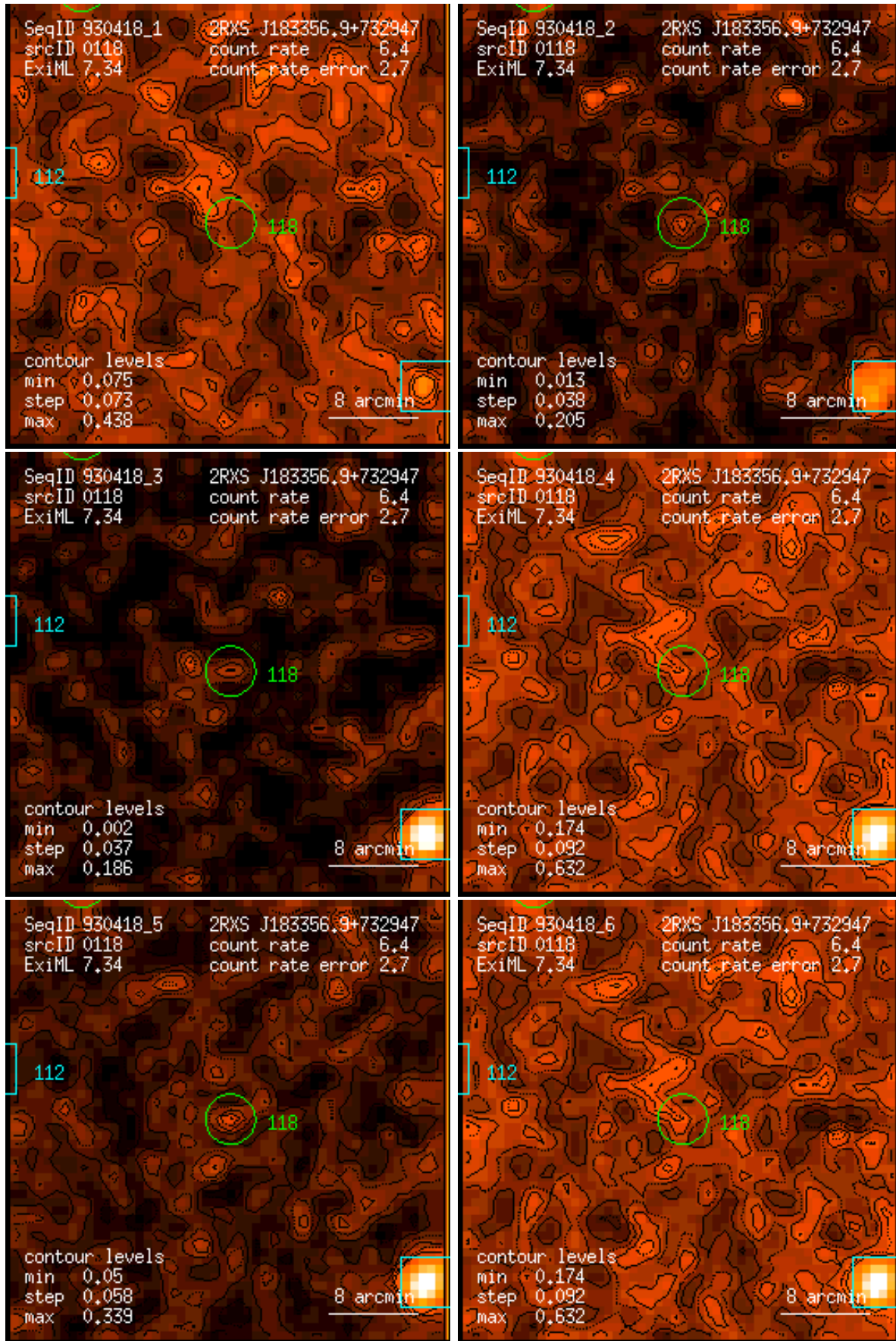
Figure 118: RASS 930418: detection 0118: band rate images, Gaussian filter: (1) PSPC channels 11 – 41, (2) 52 – 90, (3) 91 – 201, (4) 11 – 235, (5) 52 – 201, (6) 11 – 201. Broad band rates in counts/ks. Band rate contour levels in counts/ks/arcmin 2 .
