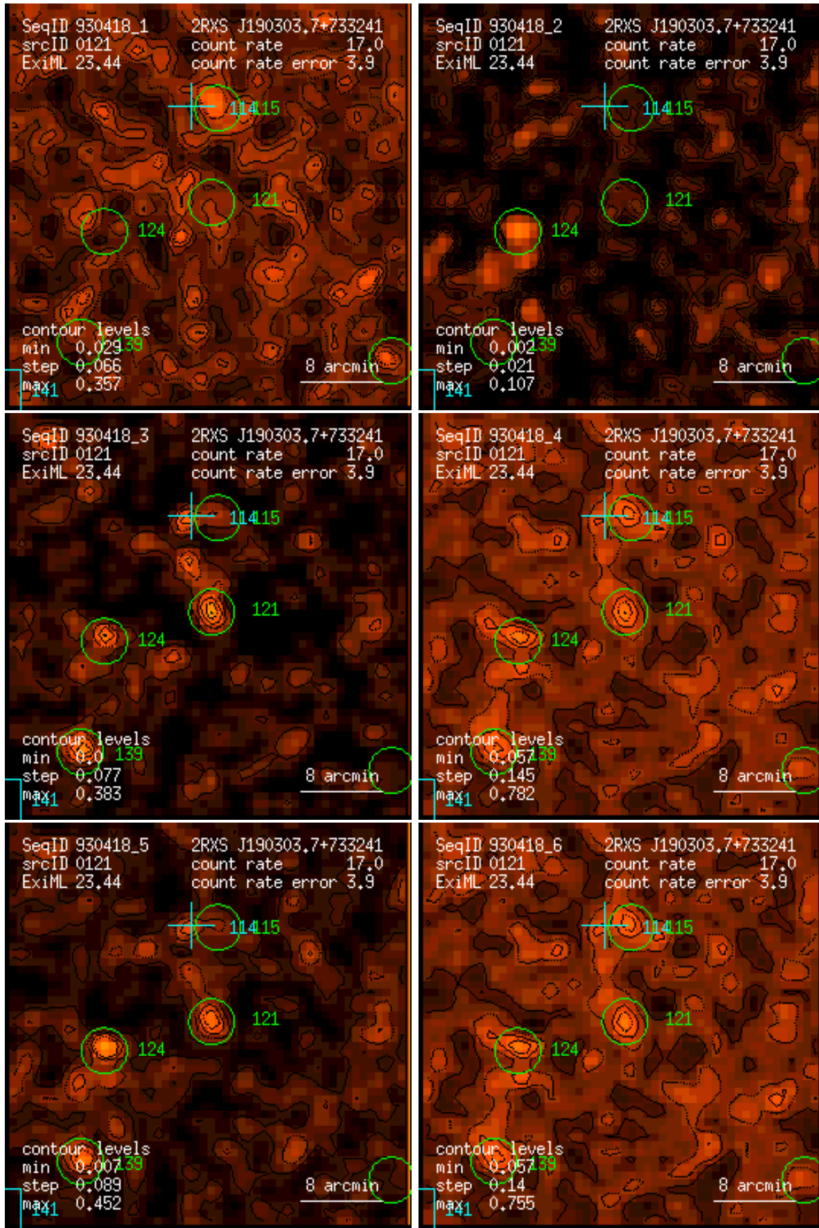
Figure 121: RASS 930418: detection 0121: band rate images, Gaussian filter: (1) PSPC channels 11 – 41, (2) 52 – 90, (3) 91 – 201, (4) 11 – 235, (5) 52 – 201, (6) 11 – 201. Broad band rates in counts/ks. Band rate contour levels in counts/ks/arcmin 2 .
