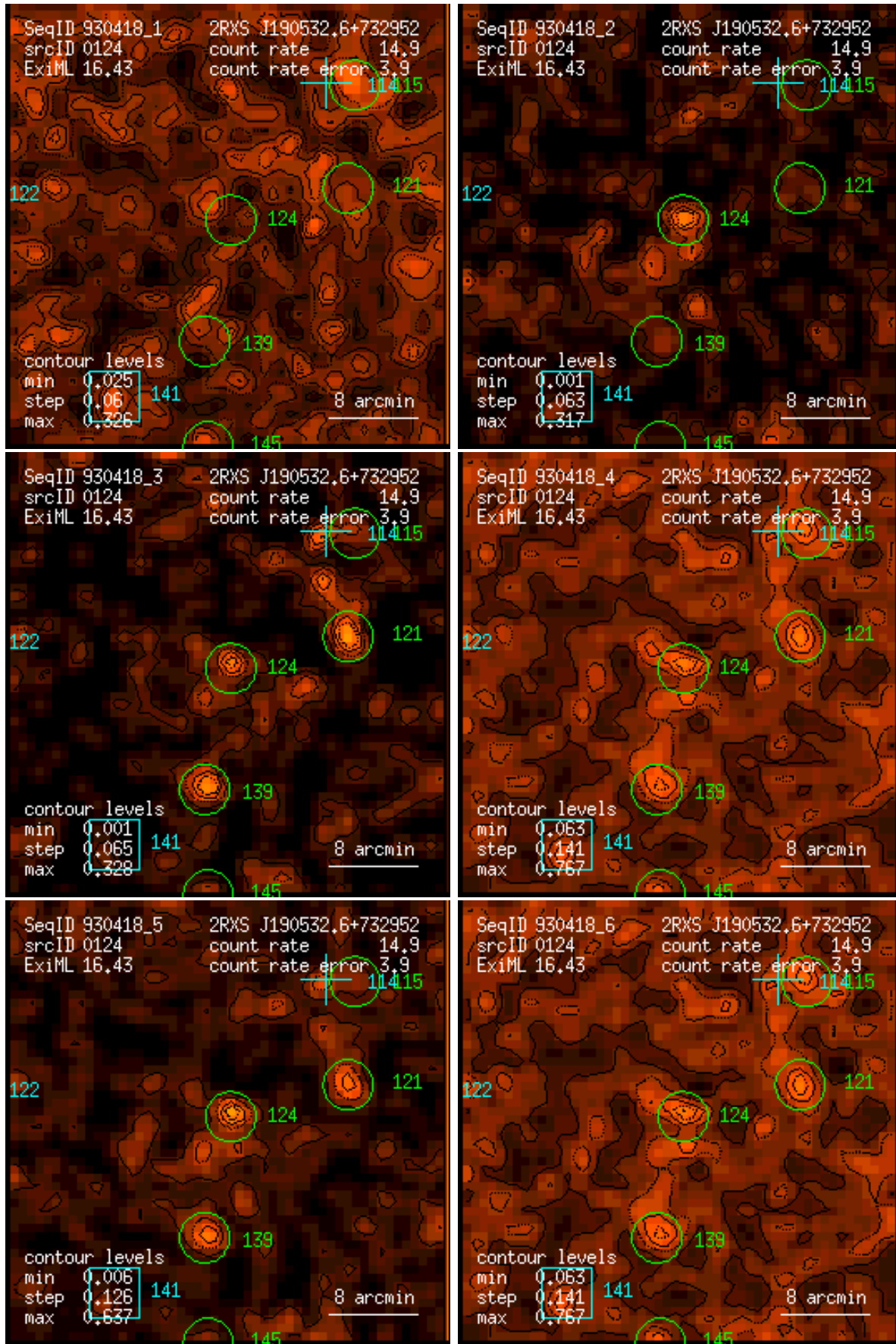
Figure 124: RASS 930418: detection 0124: band rate images, Gaussian filter: (1) PSPC channels 11 – 41, (2) 52 – 90, (3) 91 – 201, (4) 11 – 235, (5) 52 – 201, (6) 11 – 201. Broad band rates in counts/ks. Band rate contour levels in counts/ks/arcmin 2 .
