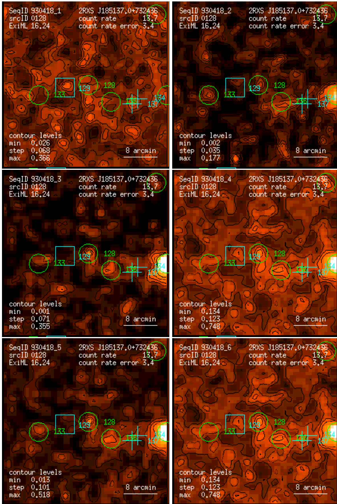
Figure 128: RASS 930418: detection 0128: band rate images, Gaussian filter: (1) PSPC channels 11 – 41, (2) 52 – 90, (3) 91 – 201, (4) 11 – 235, (5) 52 – 201, (6) 11 – 201. Broad band rates in counts/ks. Band rate contour levels in counts/ks/arcmin 2 .
