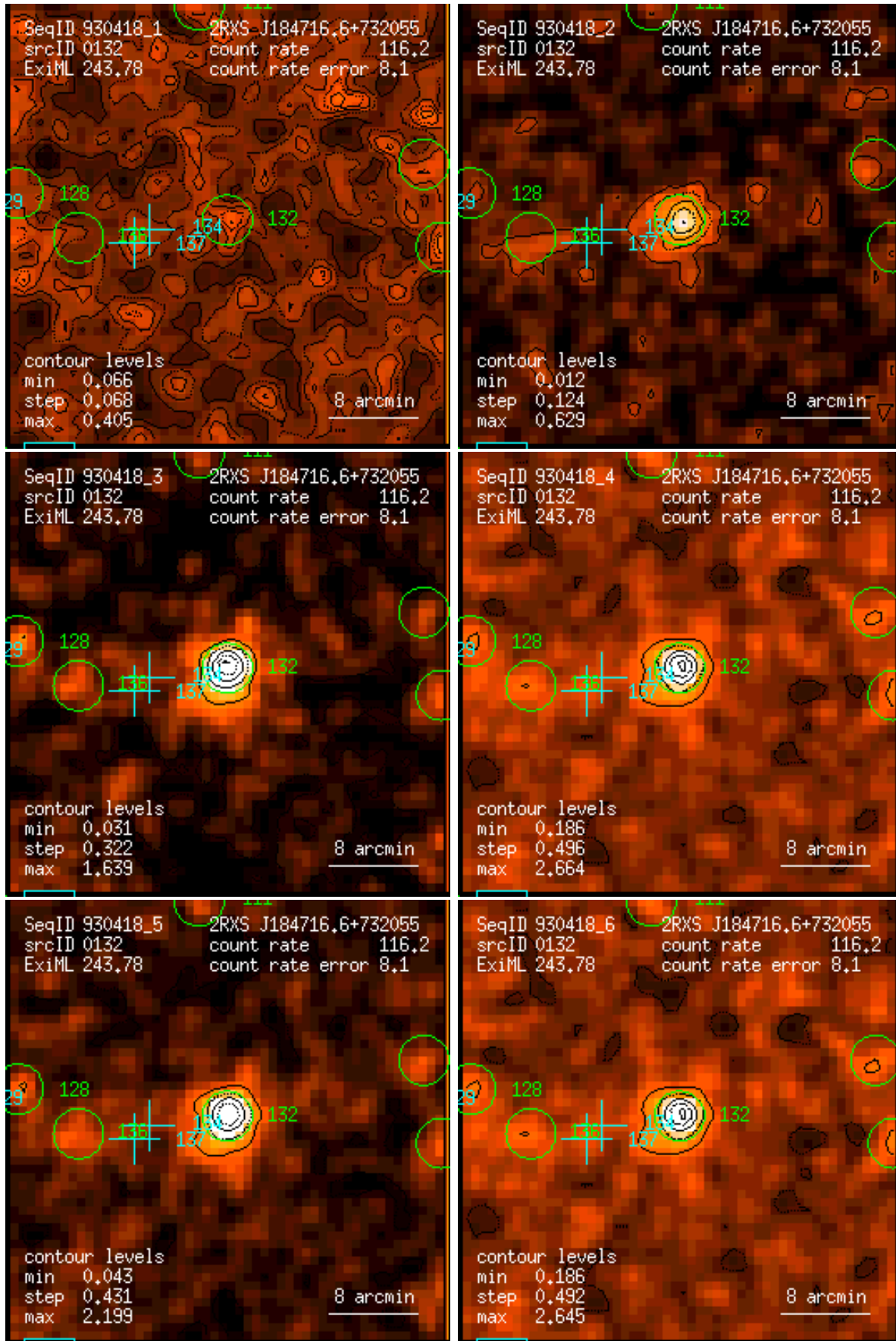
Figure 132: RASS 930418: detection 0132: band rate images, Gaussian filter: (1) PSPC channels 11 – 41, (2) 52 – 90, (3) 91 – 201, (4) 11 – 235, (5) 52 – 201, (6) 11 – 201. Broad band rates in counts/ks. Band rate contour levels in counts/ks/arcmin 2 .
