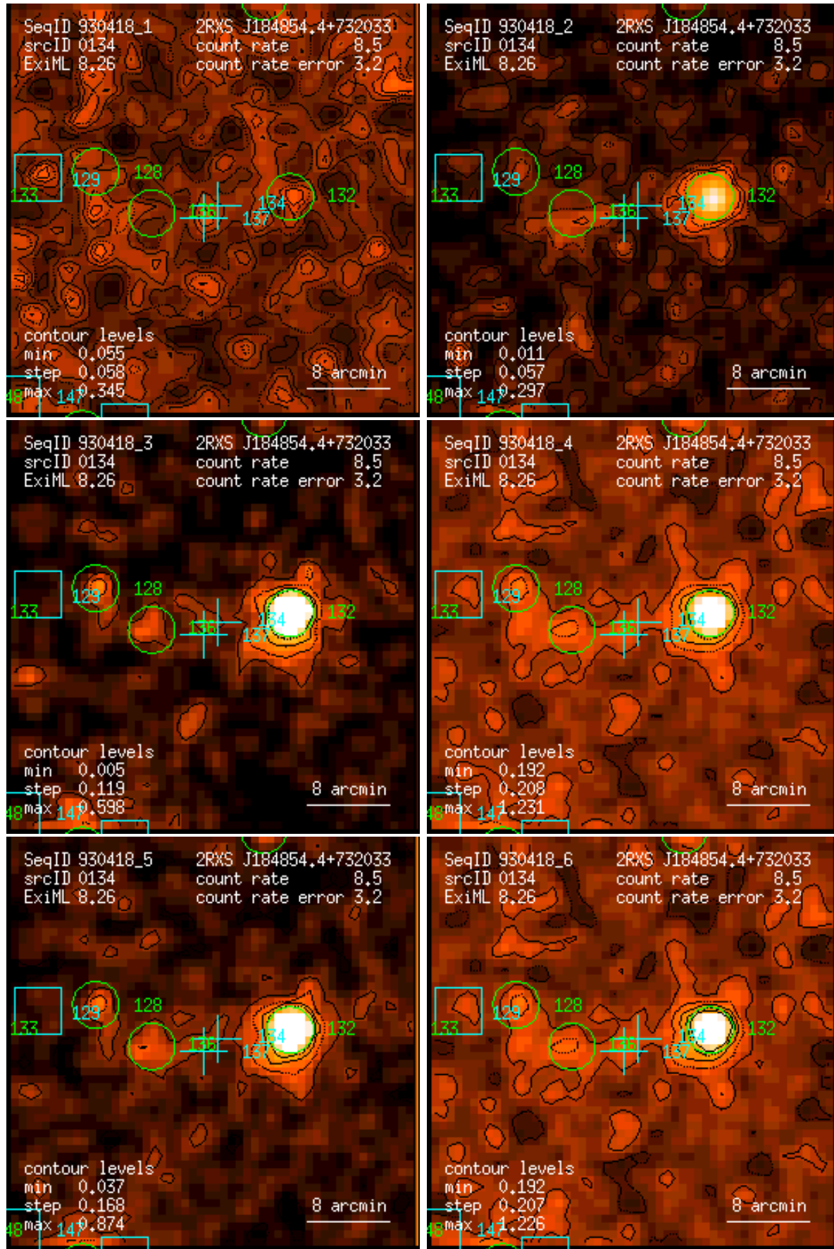
Figure 134: RASS 930418: detection 0134: band rate images, Gaussian filter: (1) PSPC channels 11 – 41, (2) 52 – 90, (3) 91 – 201, (4) 11 – 235, (5) 52 – 201, (6) 11 – 201. Broad band rates in counts/ks. Band rate contour levels in counts/ks/arcmin 2 .
