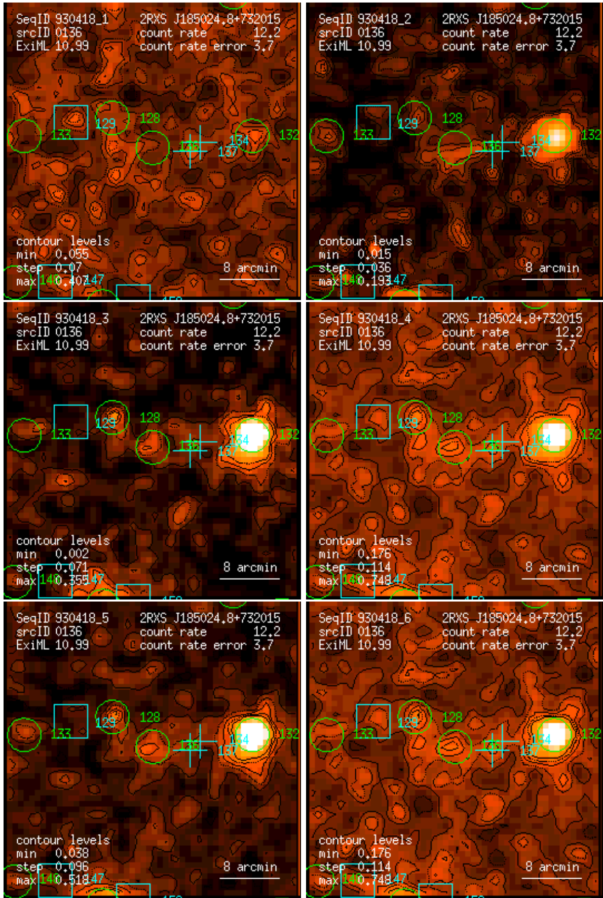
Figure 136: RASS 930418: detection 0136: band rate images, Gaussian filter: (1) PSPC channels 11 – 41, (2) 52 – 90, (3) 91 – 201, (4) 11 – 235, (5) 52 – 201, (6) 11 – 201. Broad band rates in counts/ks. Band rate contour levels in counts/ks/arcmin 2 .
