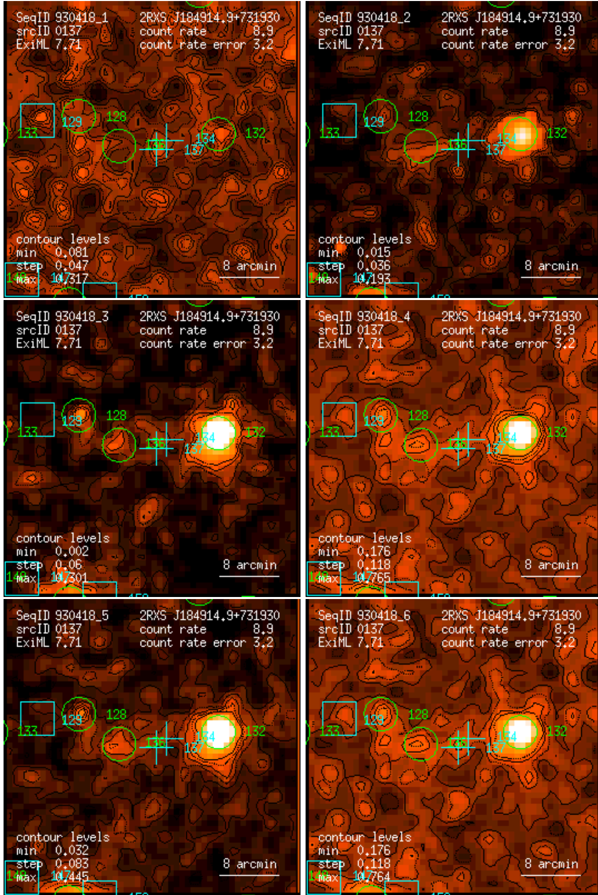
Figure 137: RASS 930418: detection 0137: band rate images, Gaussian filter: (1) PSPC channels 11 – 41, (2) 52 – 90, (3) 91 – 201, (4) 11 – 235, (5) 52 – 201, (6) 11 – 201. Broad band rates in counts/ks. Band rate contour levels in counts/ks/arcmin 2 .
