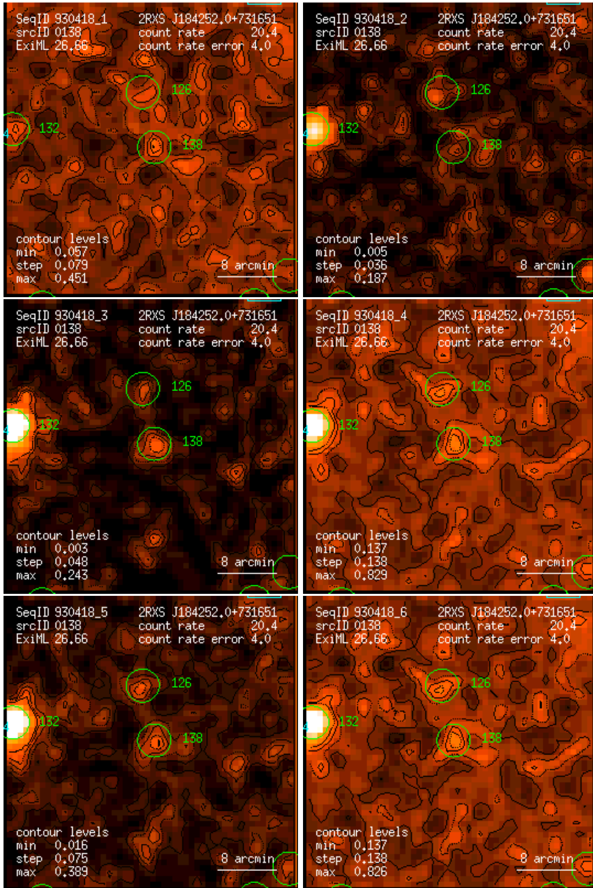
Figure 138: RASS 930418: detection 0138: band rate images, Gaussian filter: (1) PSPC channels 11 – 41, (2) 52 – 90, (3) 91 – 201, (4) 11 – 235, (5) 52 – 201, (6) 11 – 201. Broad band rates in counts/ks. Band rate contour levels in counts/ks/arcmin 2 .
