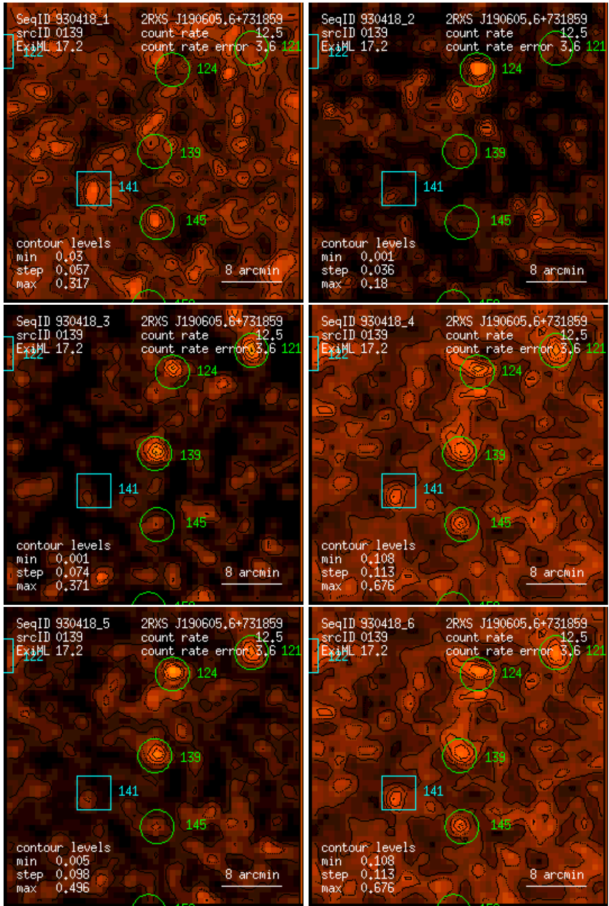
Figure 139: RASS 930418: detection 0139: band rate images, Gaussian filter: (1) PSPC channels 11 – 41, (2) 52 – 90, (3) 91 – 201, (4) 11 – 235, (5) 52 – 201, (6) 11 – 201. Broad band rates in counts/ks. Band rate contour levels in counts/ks/arcmin 2 .
