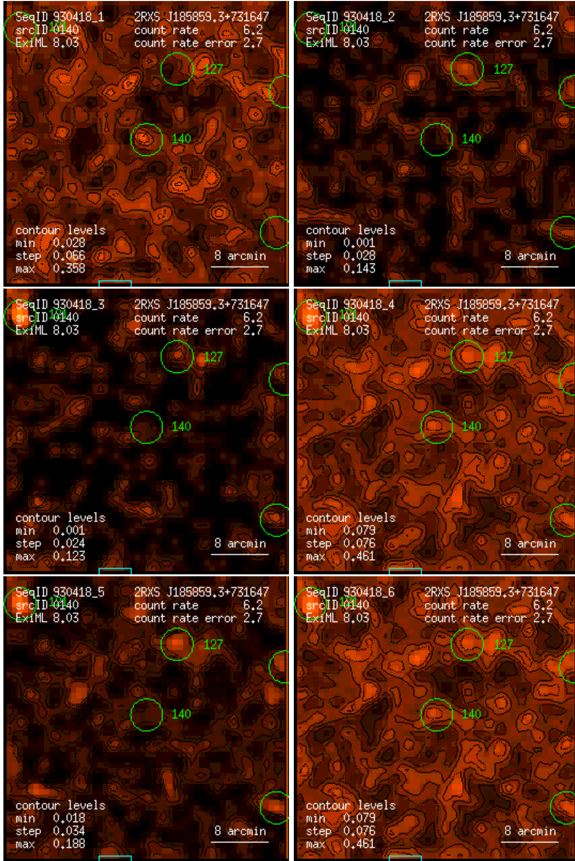
Figure 140: RASS 930418: detection 0140: band rate images, Gaussian filter: (1) PSPC channels 11 – 41, (2) 52 – 90, (3) 91 – 201, (4) 11 – 235, (5) 52 – 201, (6) 11 – 201. Broad band rates in counts/ks. Band rate contour levels in counts/ks/arcmin 2 .
