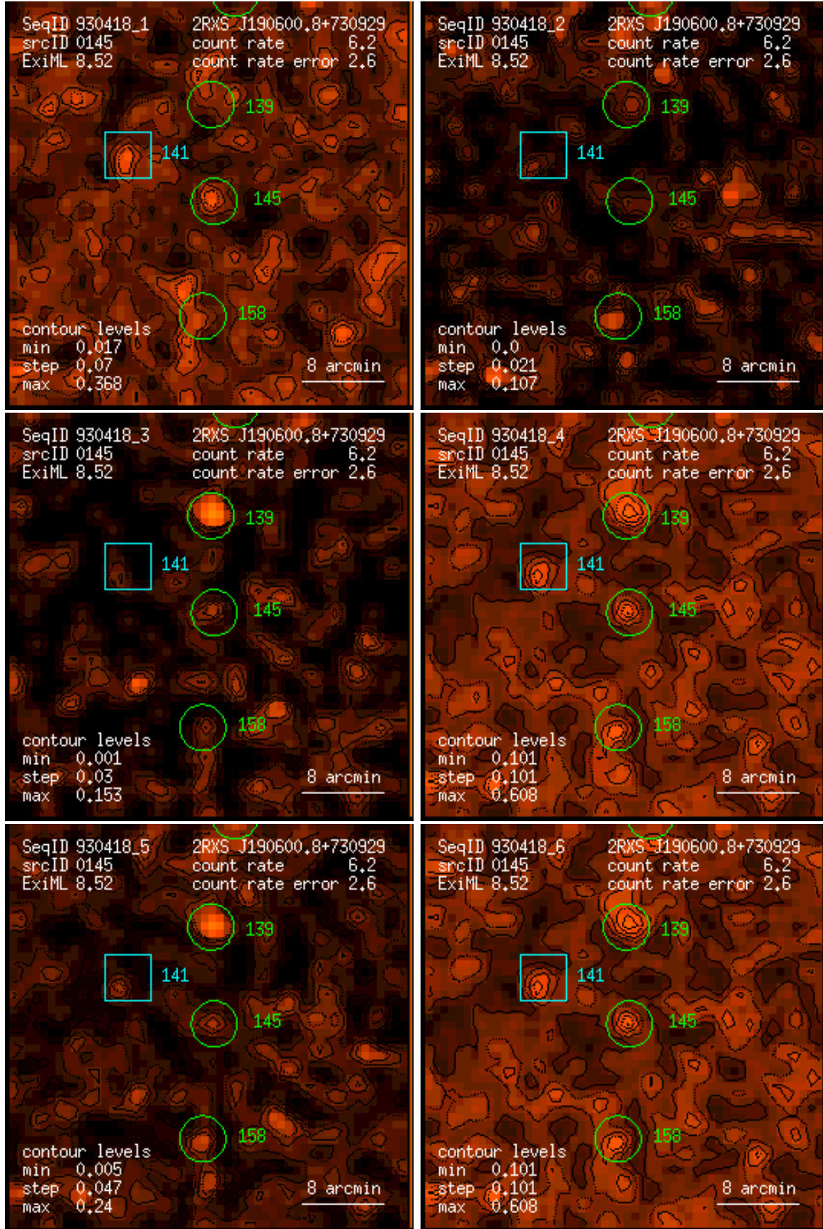
Figure 145: RASS 930418: detection 0145: band rate images, Gaussian filter: (1) PSPC channels 11 – 41, (2) 52 – 90, (3) 91 – 201, (4) 11 – 235, (5) 52 – 201, (6) 11 – 201. Broad band rates in counts/ks. Band rate contour levels in counts/ks/arcmin 2 .
