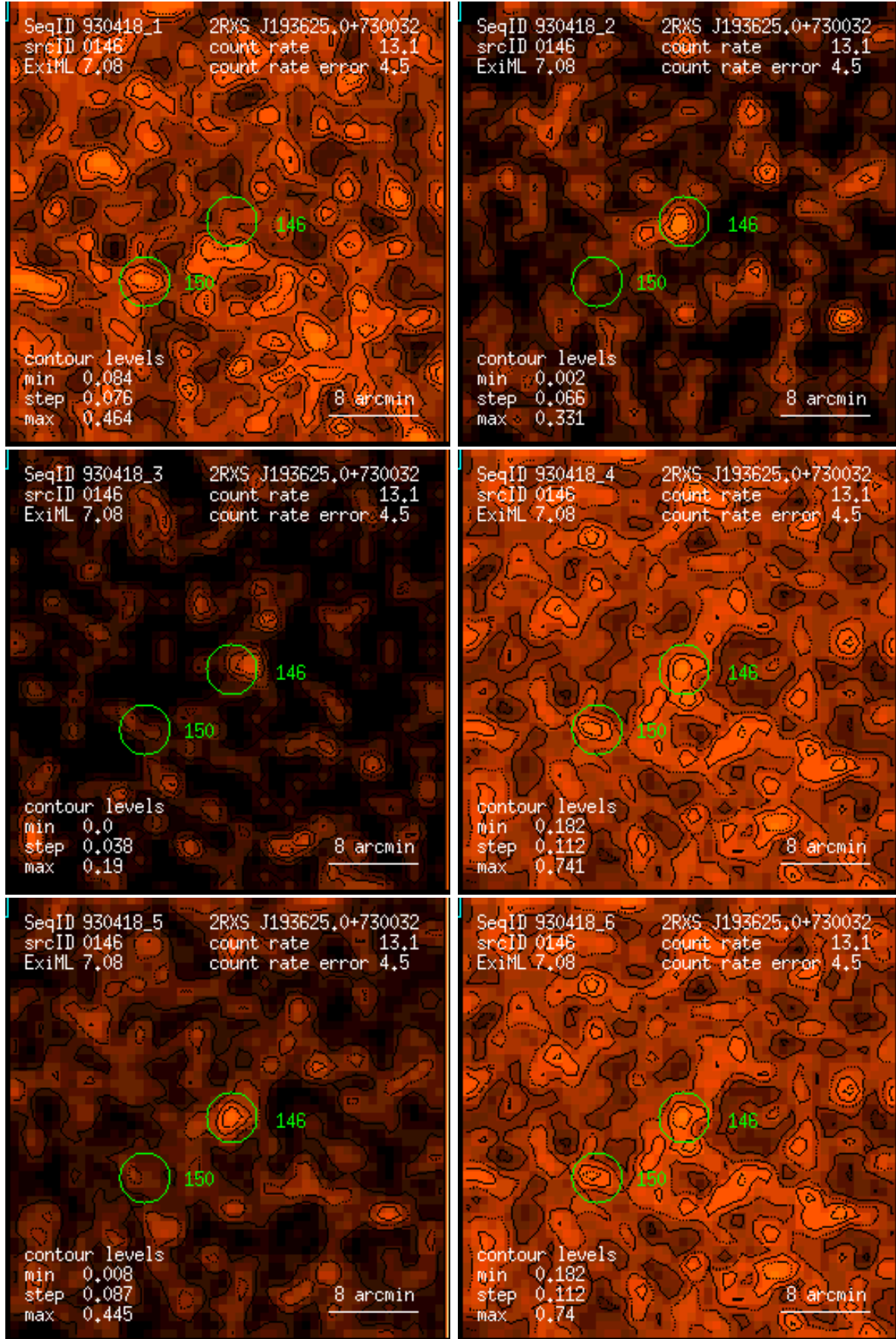
Figure 146: RASS 930418: detection 0146: band rate images, Gaussian filter: (1) PSPC channels 11 – 41, (2) 52 – 90, (3) 91 – 201, (4) 11 – 235, (5) 52 – 201, (6) 11 – 201. Broad band rates in counts/ks. Band rate contour levels in counts/ks/arcmin 2 .
