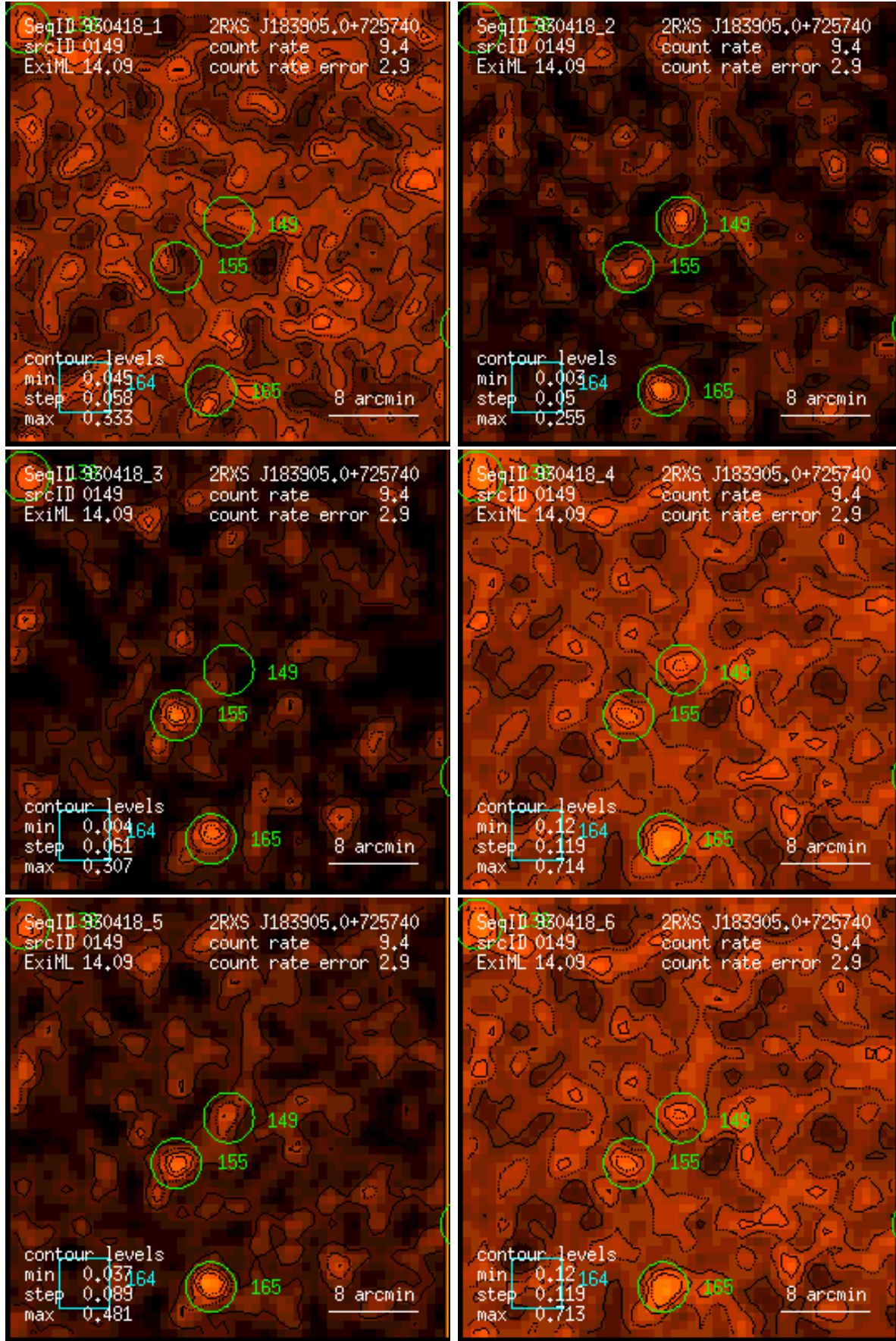
Figure 149: RASS 930418: detection 0149: band rate images, Gaussian filter: (1) PSPC channels 11 – 41, (2) 52 – 90, (3) 91 – 201, (4) 11 – 235, (5) 52 – 201, (6) 11 – 201. Broad band rates in counts/ks. Band rate contour levels in counts/ks/arcmin 2 .
