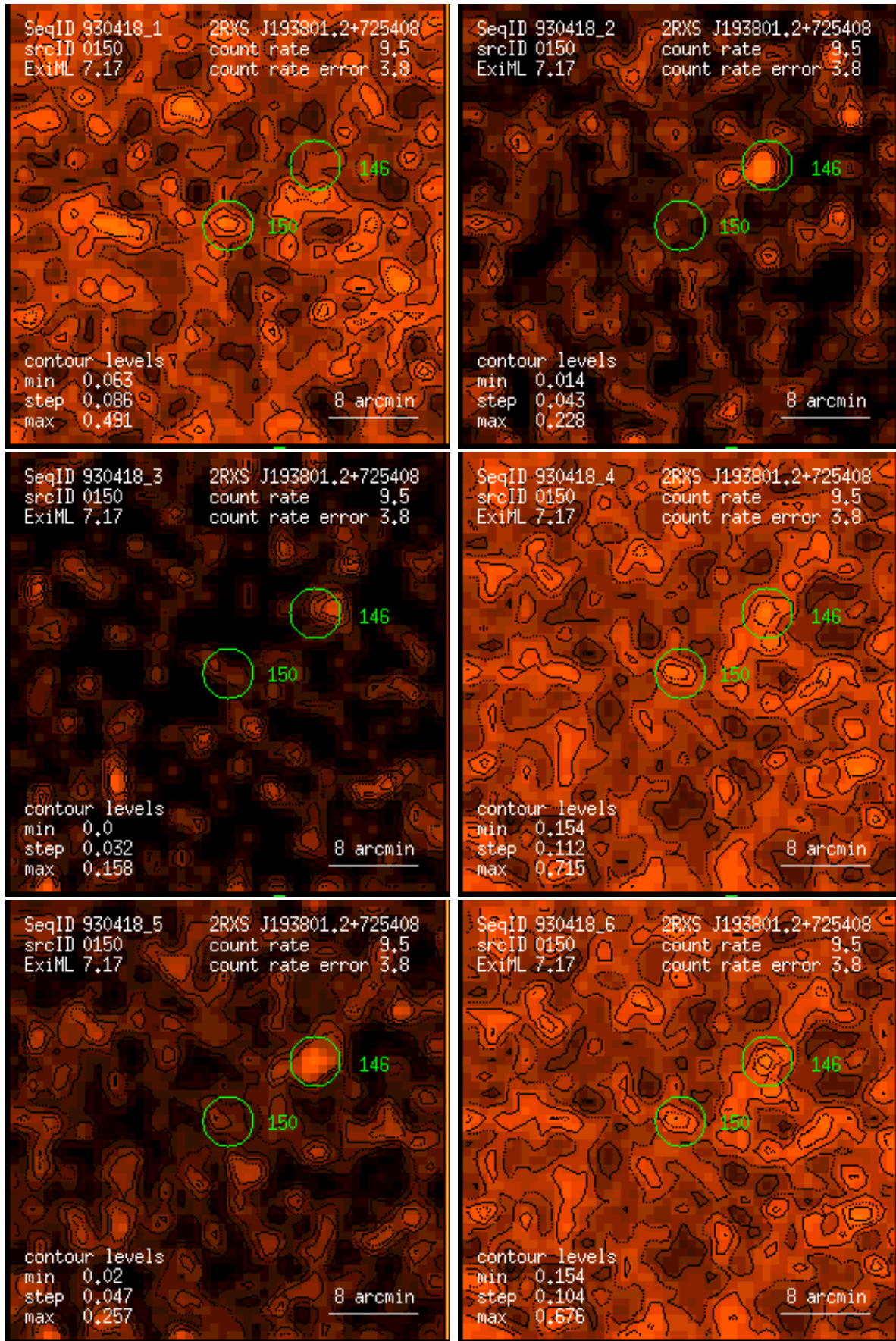
Figure 150: RASS 930418: detection 0150: band rate images, Gaussian filter: (1) PSPC channels 11 – 41, (2) 52 – 90, (3) 91 – 201, (4) 11 – 235, (5) 52 – 201, (6) 11 – 201. Broad band rates in counts/ks. Band rate contour levels in counts/ks/arcmin 2 .
