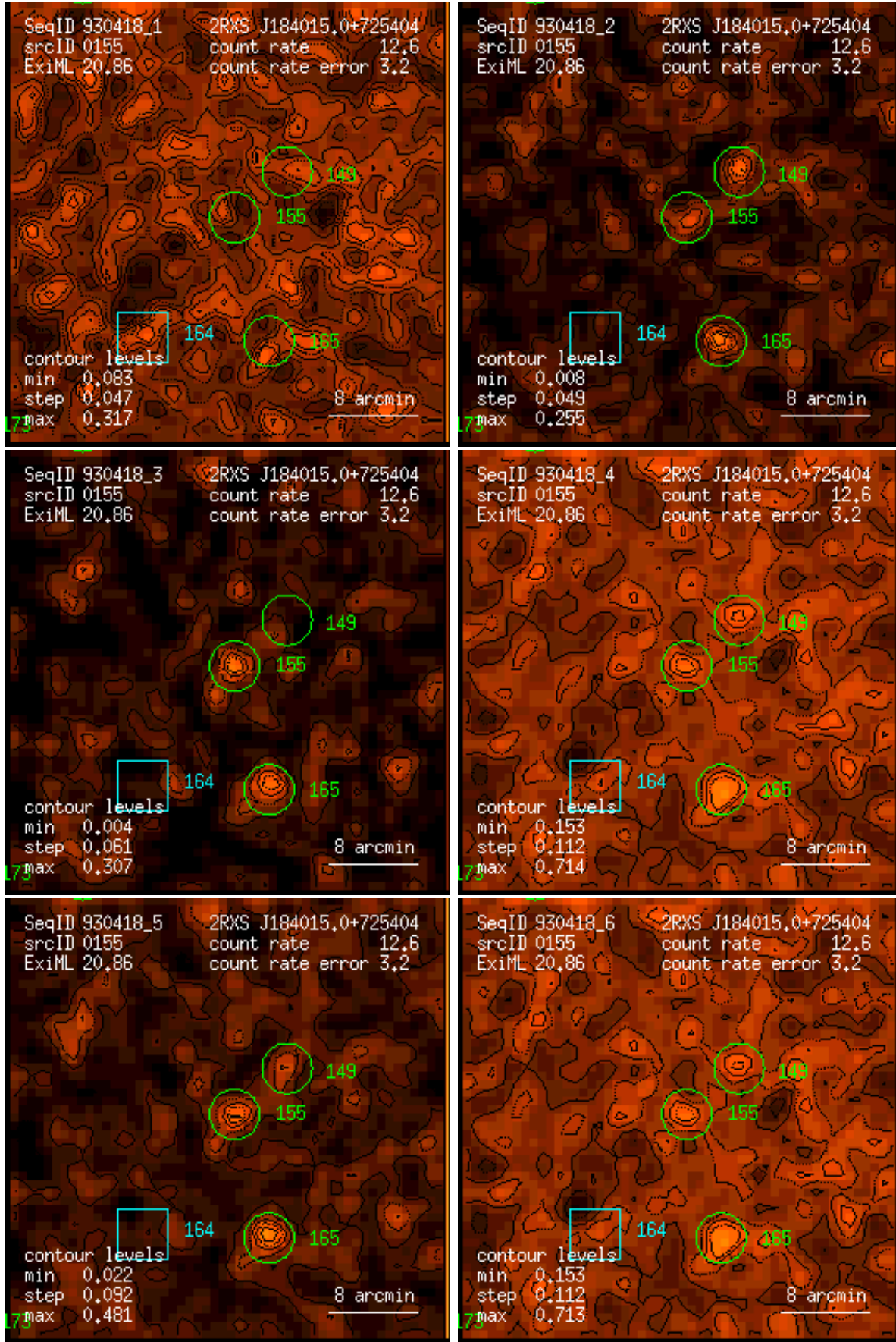
Figure 155: RASS 930418: detection 0155: band rate images, Gaussian filter: (1) PSPC channels 11 – 41, (2) 52 – 90, (3) 91 – 201, (4) 11 – 235, (5) 52 – 201, (6) 11 – 201. Broad band rates in counts/ks. Band rate contour levels in counts/ks/arcmin 2 .
