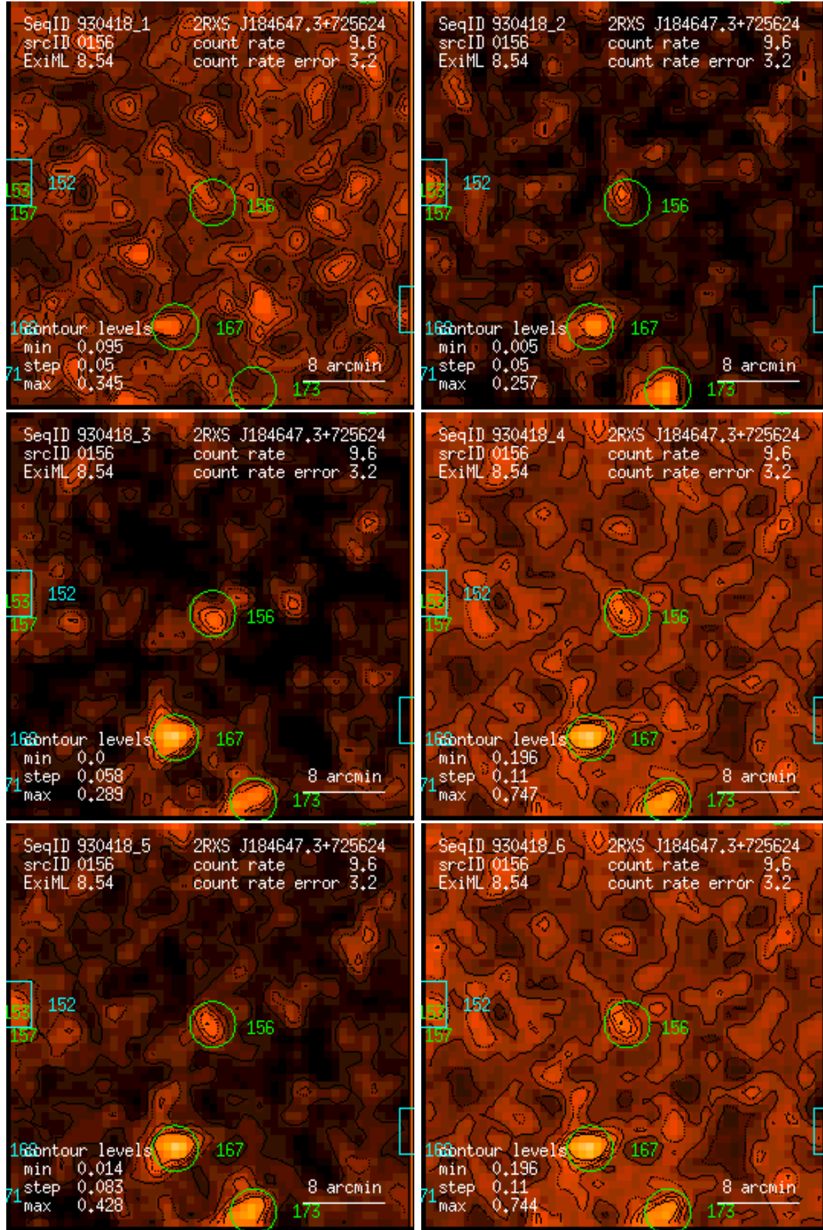
Figure 156: RASS 930418: detection 0156: band rate images, Gaussian filter: (1) PSPC channels 11 – 41, (2) 52 – 90, (3) 91 – 201, (4) 11 – 235, (5) 52 – 201, (6) 11 – 201. Broad band rates in counts/ks. Band rate contour levels in counts/ks/arcmin 2 .
