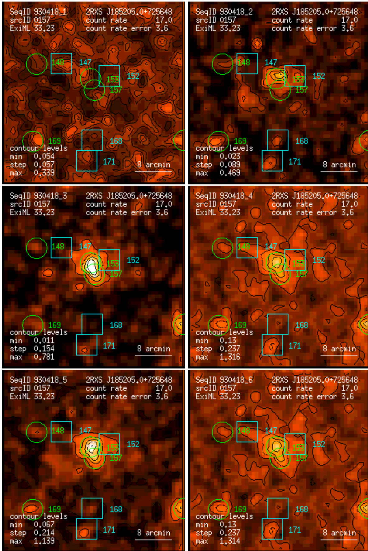
Figure 157: RASS 930418: detection 0157: band rate images, Gaussian filter: (1) PSPC channels 11 – 41, (2) 52 – 90, (3) 91 – 201, (4) 11 – 235, (5) 52 – 201, (6) 11 – 201. Broad band rates in counts/ks. Band rate contour levels in counts/ks/arcmin 2 .
