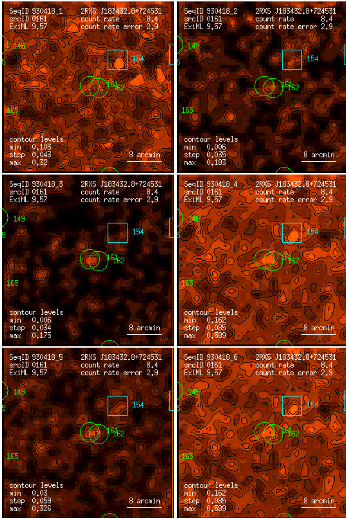
Figure 161: RASS 930418: detection 0161: band rate images, Gaussian filter: (1) PSPC channels 11 – 41, (2) 52 – 90, (3) 91 – 201, (4) 11 – 235, (5) 52 – 201, (6) 11 – 201. Broad band rates in counts/ks. Band rate contour levels in counts/ks/arcmin 2 .
