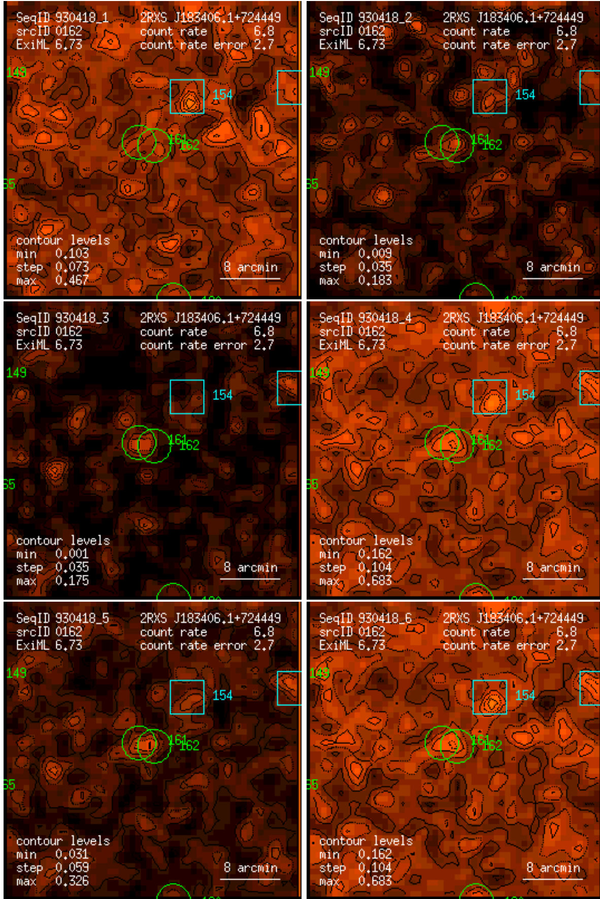
Figure 162: RASS 930418: detection 0162: band rate images, Gaussian filter: (1) PSPC channels 11 – 41, (2) 52 – 90, (3) 91 – 201, (4) 11 – 235, (5) 52 – 201, (6) 11 – 201. Broad band rates in counts/ks. Band rate contour levels in counts/ks/arcmin 2 .
