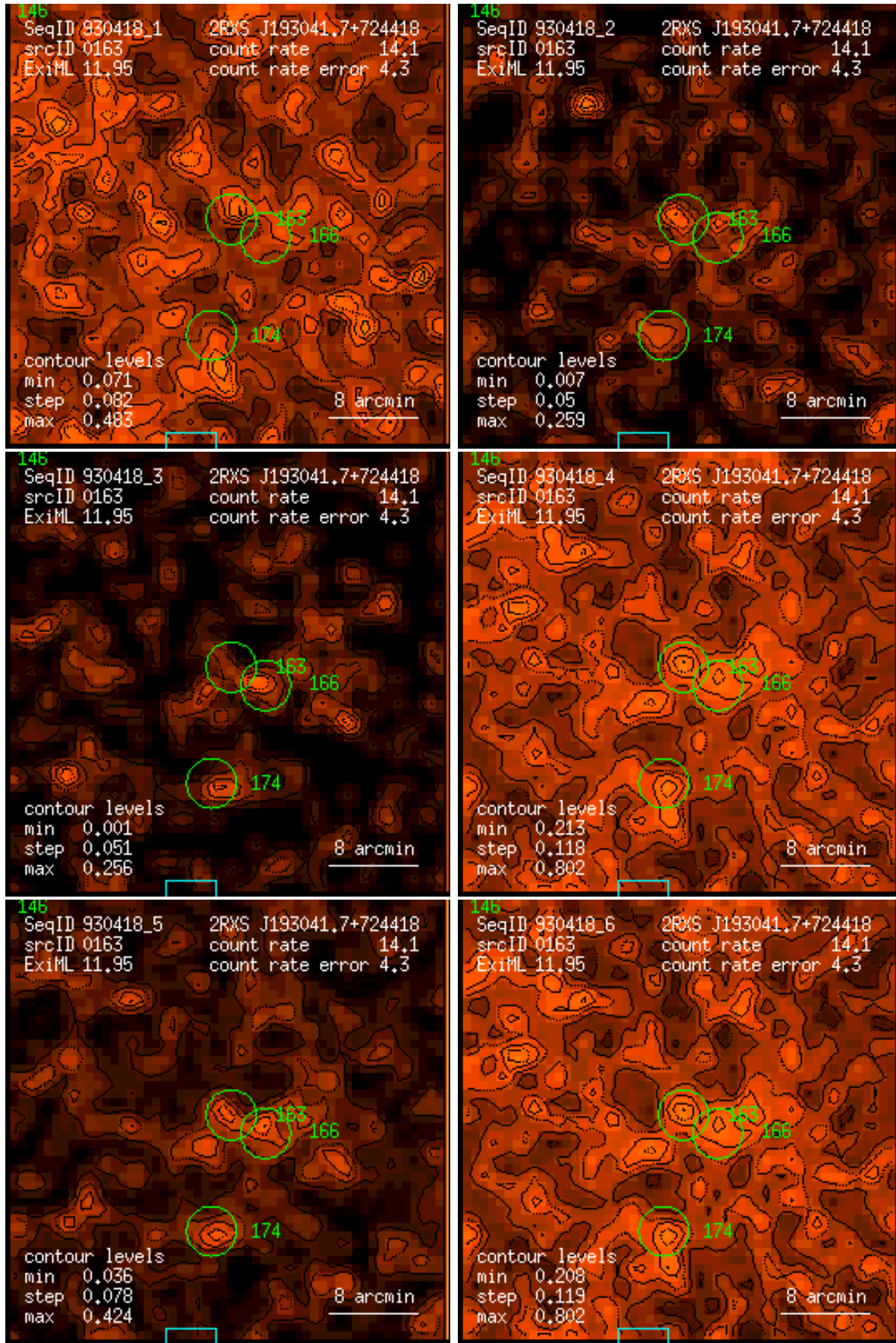
Figure 163: RASS 930418: detection 0163: band rate images, Gaussian filter: (1) PSPC channels 11 – 41, (2) 52 – 90, (3) 91 – 201, (4) 11 – 235, (5) 52 – 201, (6) 11 – 201. Broad band rates in counts/ks. Band rate contour levels in counts/ks/arcmin 2 .
