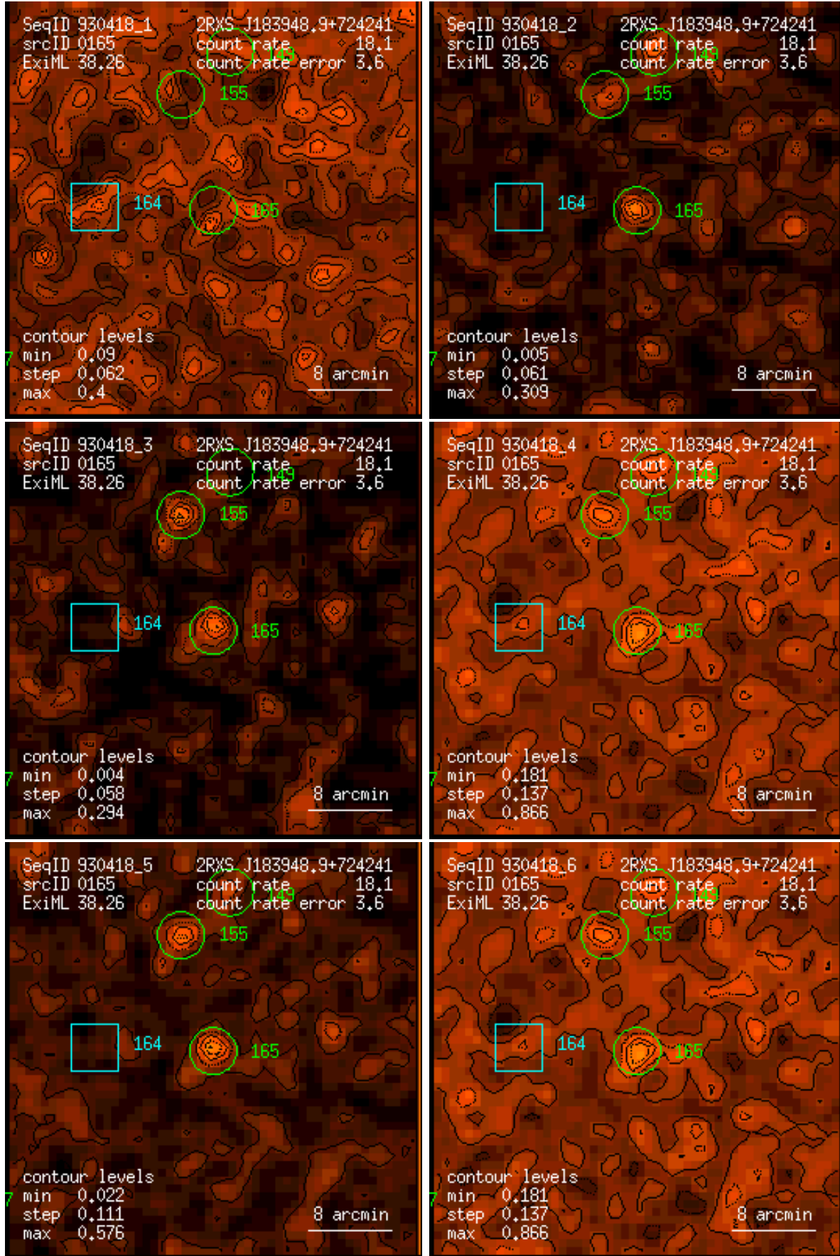
Figure 165: RASS 930418: detection 0165: band rate images, Gaussian filter: (1) PSPC channels 11 – 41, (2) 52 – 90, (3) 91 – 201, (4) 11 – 235, (5) 52 – 201, (6) 11 – 201. Broad band rates in counts/ks. Band rate contour levels in counts/ks/arcmin 2 .
