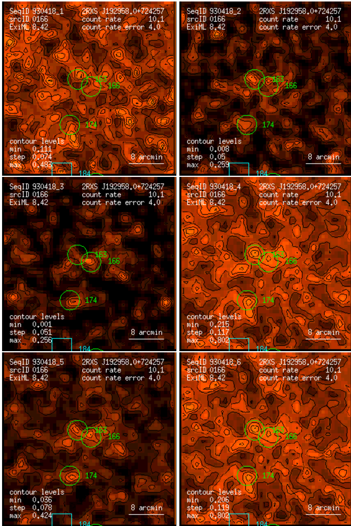
Figure 166: RASS 930418: detection 0166: band rate images, Gaussian filter: (1) PSPC channels 11 – 41, (2) 52 – 90, (3) 91 – 201, (4) 11 – 235, (5) 52 – 201, (6) 11 – 201. Broad band rates in counts/ks. Band rate contour levels in counts/ks/arcmin 2 .
