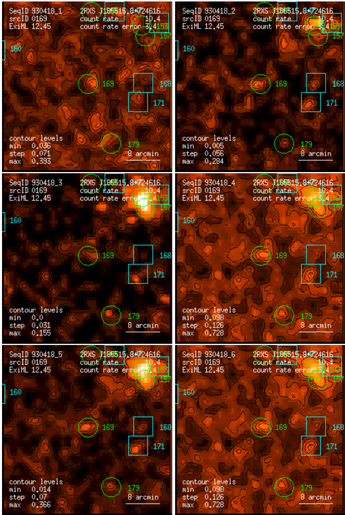
Figure 169: RASS 930418: detection 0169: band rate images, Gaussian filter: (1) PSPC channels 11 – 41, (2) 52 – 90, (3) 91 – 201, (4) 11 – 235, (5) 52 – 201, (6) 11 – 201. Broad band rates in counts/ks. Band rate contour levels in counts/ks/arcmin 2 .
