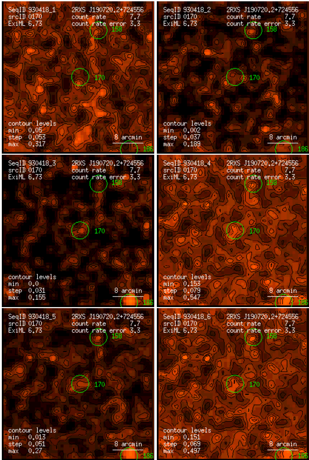
Figure 170: RASS 930418: detection 0170: band rate images, Gaussian filter: (1) PSPC channels 11 – 41, (2) 52 – 90, (3) 91 – 201, (4) 11 – 235, (5) 52 – 201, (6) 11 – 201. Broad band rates in counts/ks. Band rate contour levels in counts/ks/arcmin 2 .
