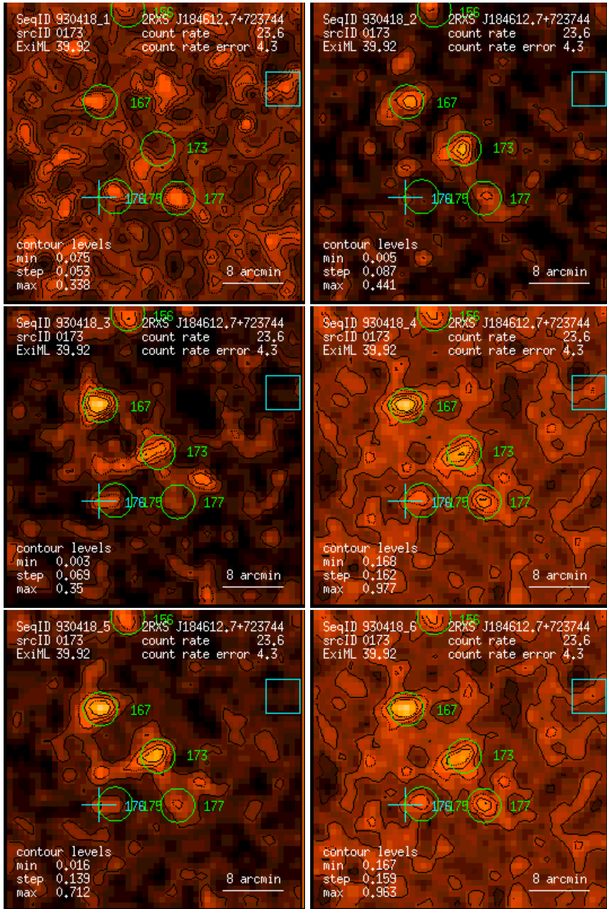
Figure 173: RASS 930418: detection 0173: band rate images, Gaussian filter: (1) PSPC channels 11 – 41, (2) 52 – 90, (3) 91 – 201, (4) 11 – 235, (5) 52 – 201, (6) 11 – 201. Broad band rates in counts/ks. Band rate contour levels in counts/ks/arcmin 2 .
